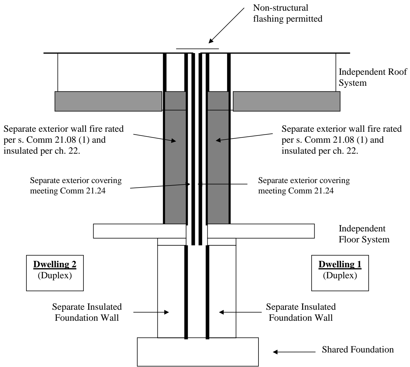
Detail A
