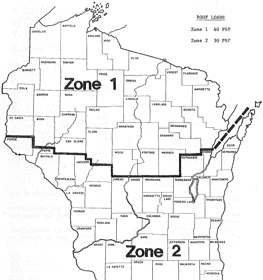
ZONE MAP FOR ROOF LOADS
