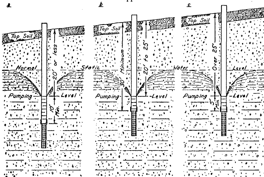
Figure A-1. Construction of Wells in Sand and Gravel with Screens, by Percussion Equipment. See Table I, a.
