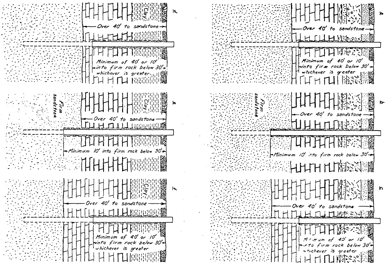
Figure A-25. Construction of Wells Terminating in Sandstone Underlying Limestone extending to a depth greater than 40 feet with or without Unconsolidated Overburden over the Limestone, by either Percussion or Rotary Equipment. See Table 1, q.
