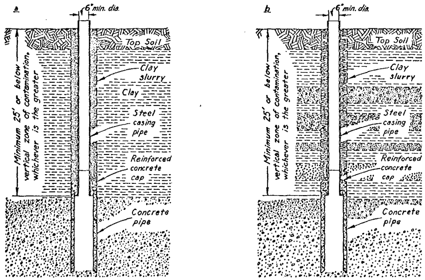
Figure 2. Bored Type Well Construction. See NR 112.09.
