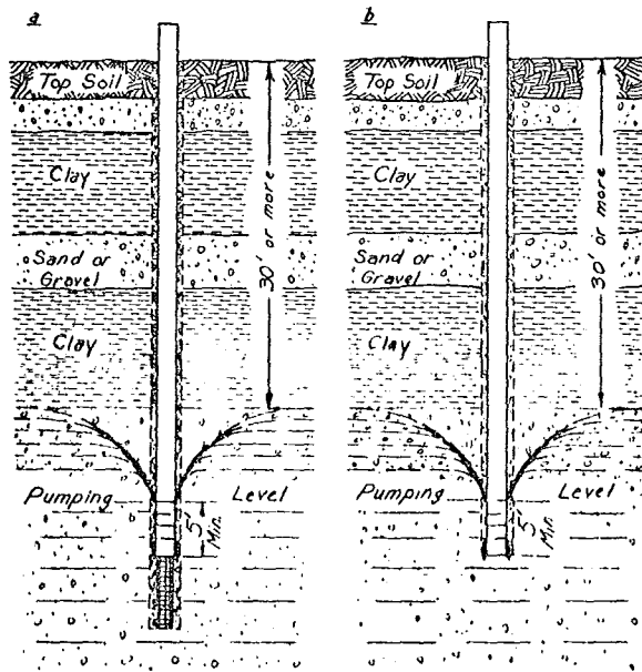
Figure A-6. Construction of Wells Terminating in Sand and Gravel Underlying Clay or Similar Material containing layers of Sand and Gravel, with and without Screens, by Rotary Equipment. See Table I, b.
