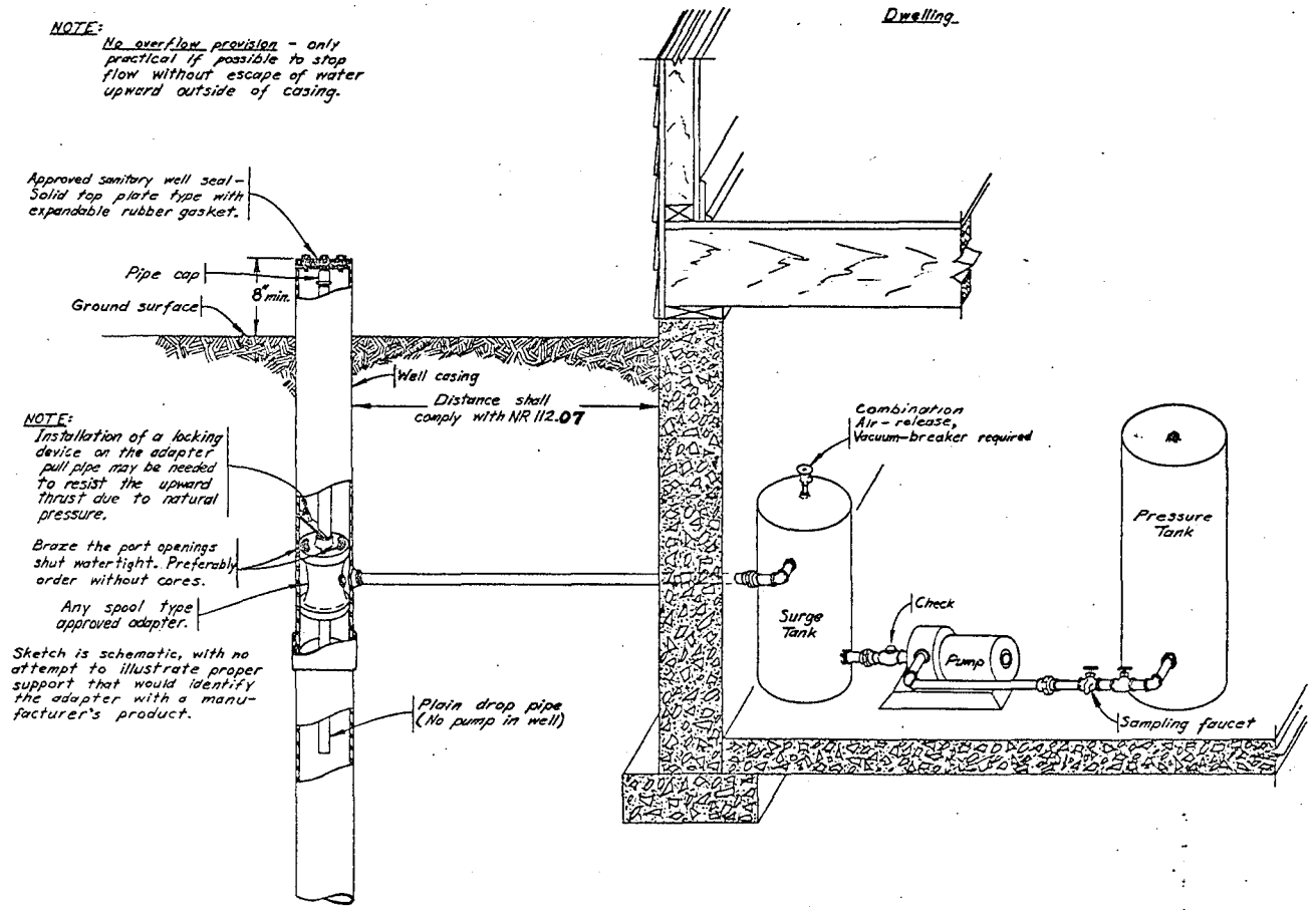
Figure 19. Pump Installation for Flowing Artesian Well using an Approved Pitless Adapter, Surge Tank and Booster Pump with no Overflow Provision.
