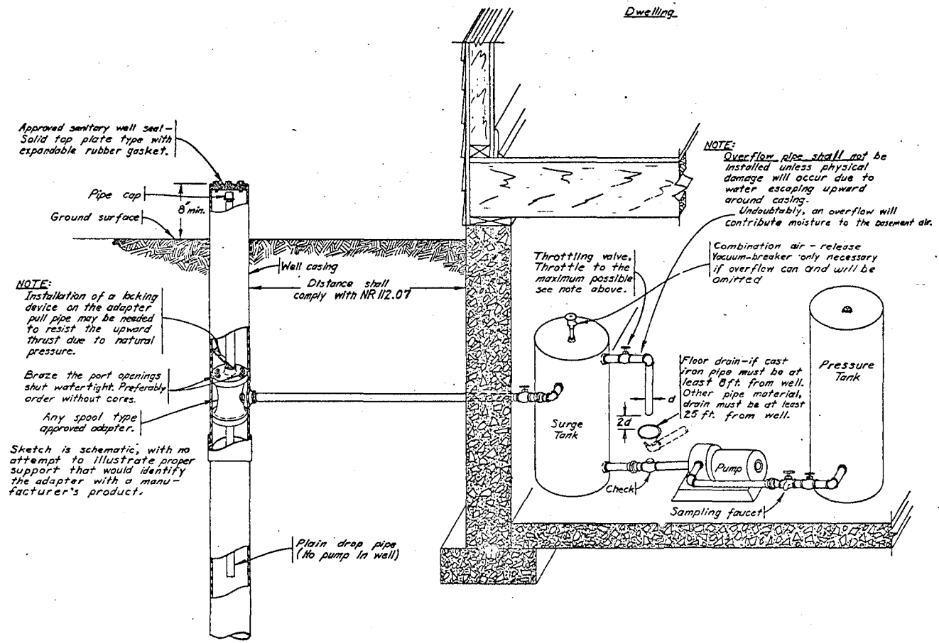
Figure 23. Pump Installation for Flowing Well Using an Approved Pitless Adapter, Surge Tank and Booster Pump, with Overflow Provision off the Surge Tank, if necessary.
