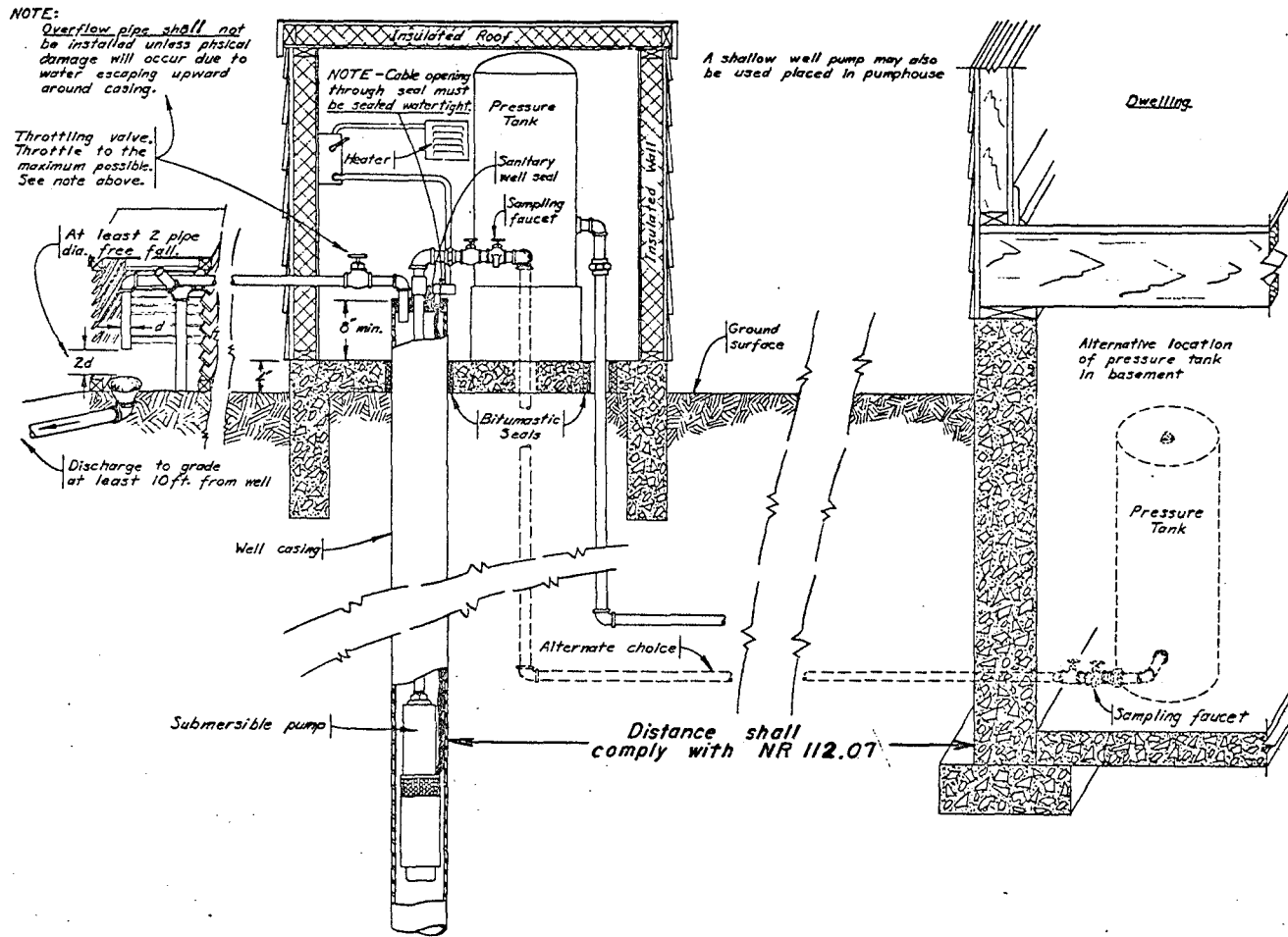
Figure 20. Pump Installation for Flowing Well using Submersible Pump and Above-Ground Discharge and Overflow Provision, if necessary.
