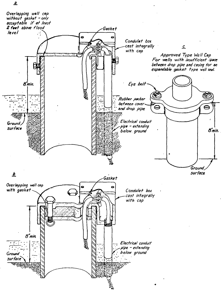
Figure 10. Types of Well Seals. (a) overlapping well cap with skirted sides. (b) and (c) seals using compressible rubber gaskets. See NR 112.17(2) and (4).
