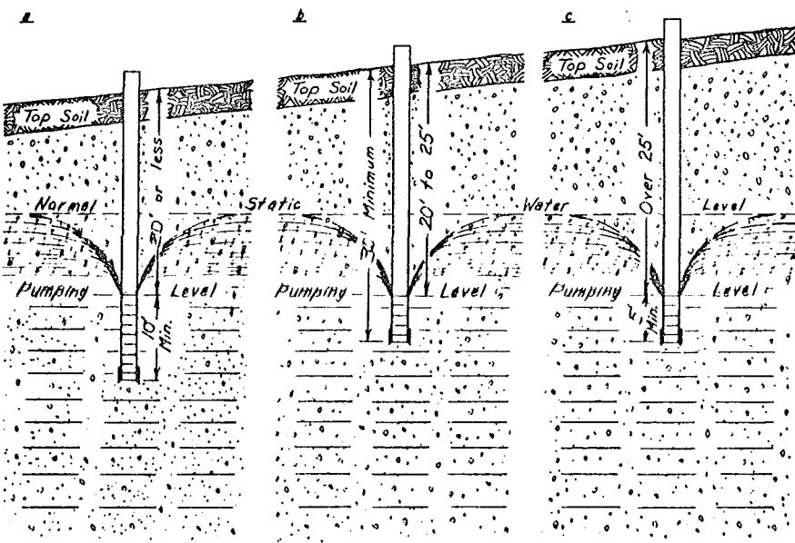
Figure A-2. Construction of Wells in Sand and Gravel without Screens, by Percussion Equipment. See Table I, a.
