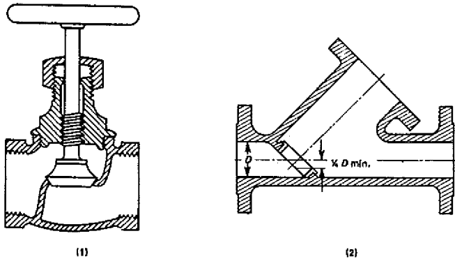
FIG. 122.1.7(C) TYPICAL GLOBE VALVES
