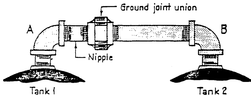
Figure 10.473-3 Detail of the cross connection which can be used in Figure 10.473-2.
