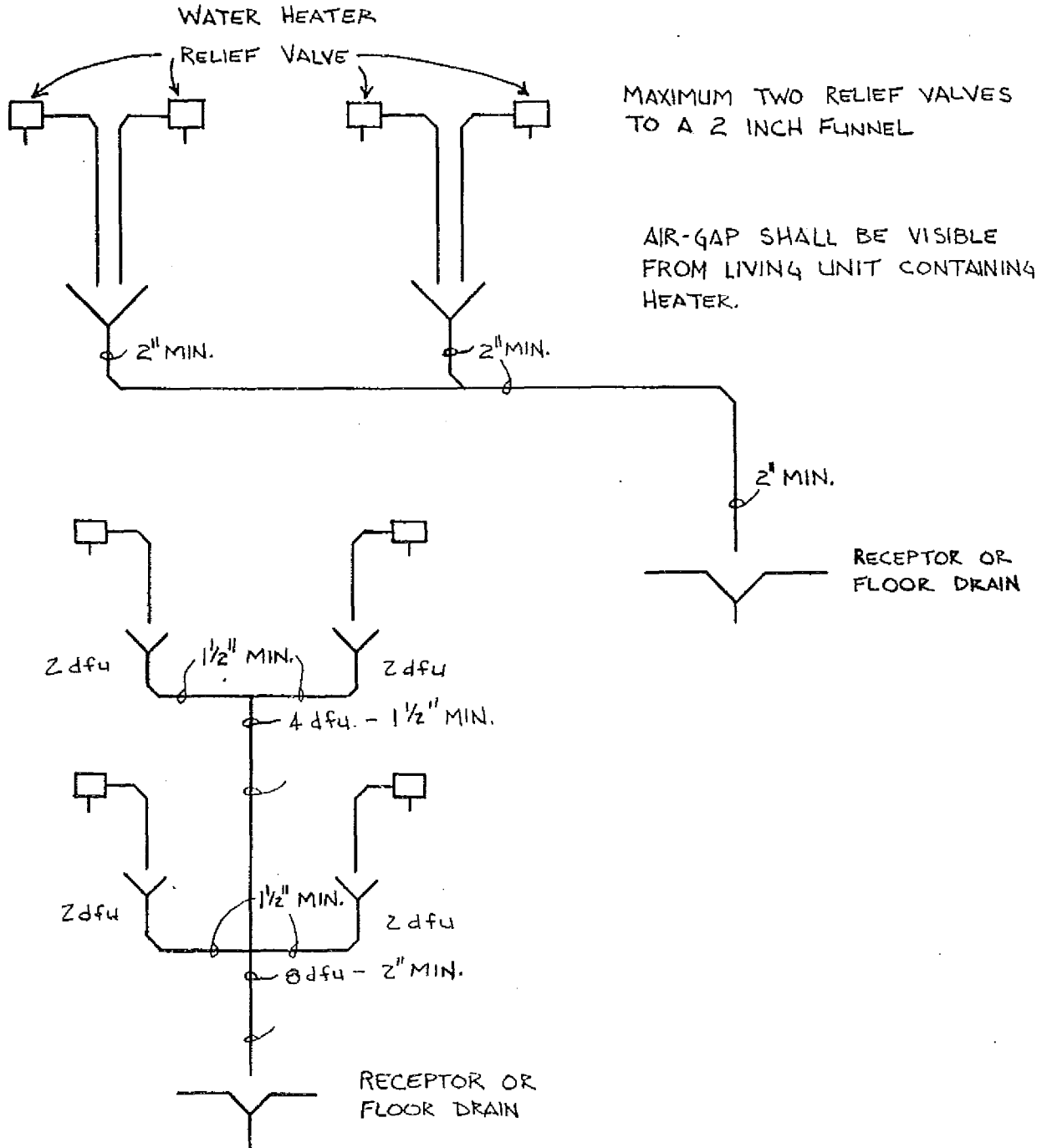
LOCAL WASTE PIPES SERVING WATER HEATER RELIEF VALVES.
