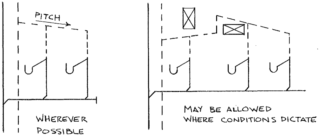
A-82.31 (15) (a) VENT GRADES AND CONNECTIONS.
