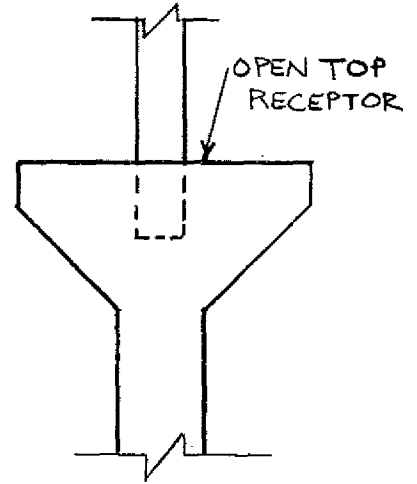
AIR BREAK
