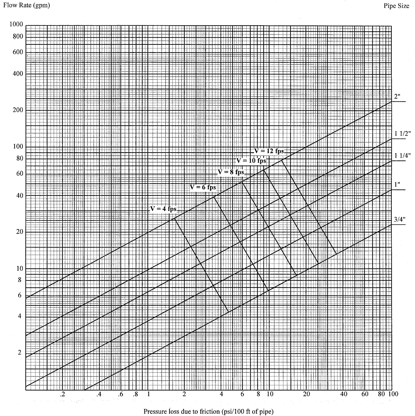
Graph A-382.40 (7)-7 PRESSURE LOSSES DUE TO FLOW FRICTION Material: Polyethylene Tubing, Copper Tube Size, ASTM D2737; (C = 150)
