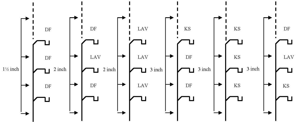
Most restrictive fixture determines stack size
