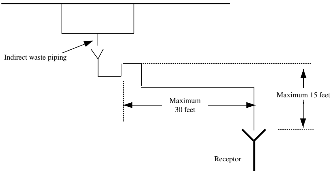
MAXIMUM LENGTH OF LOCAL WASTE PIPE
