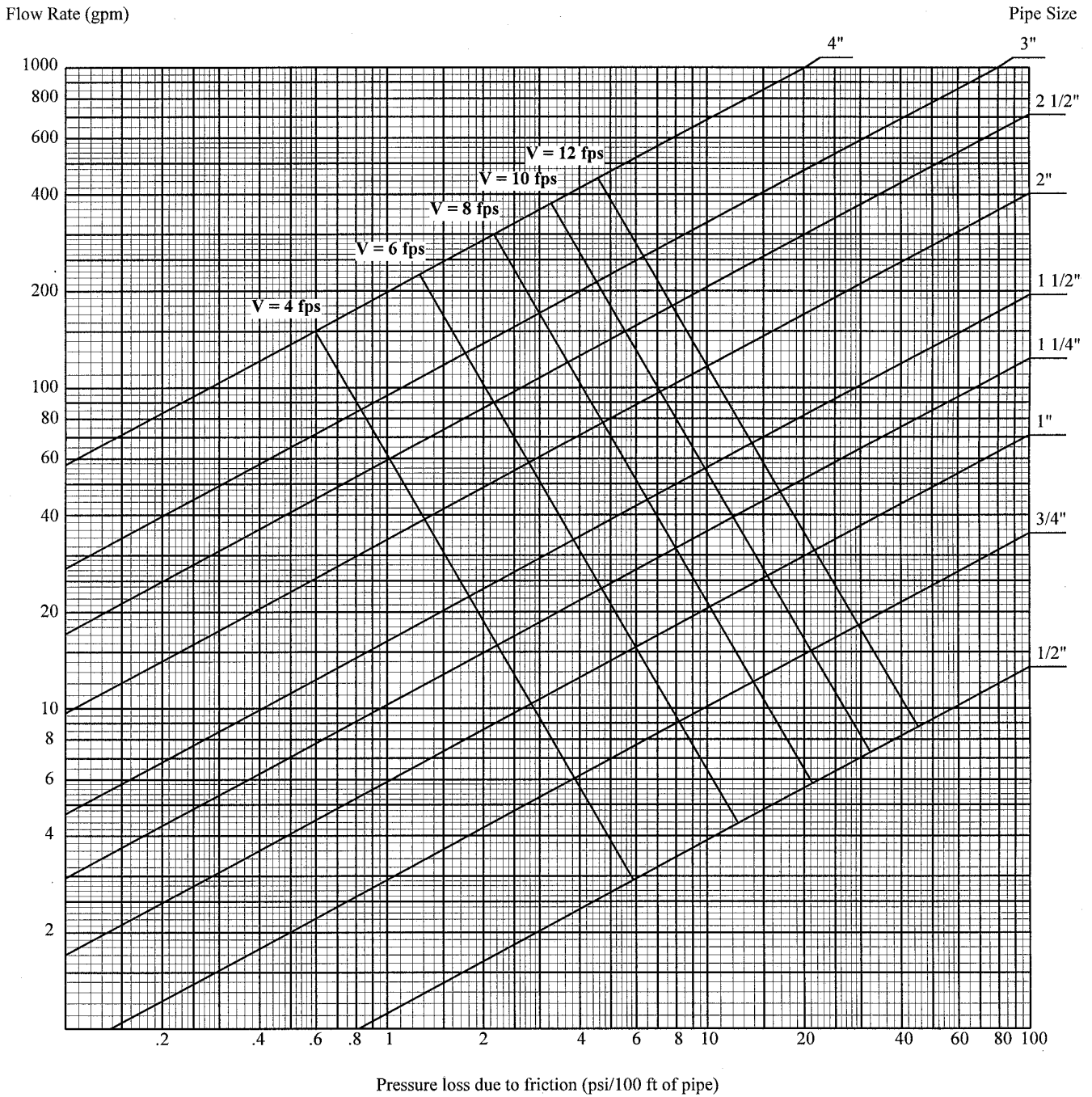
Graph A-382.40 (7)-3 PRESSURE LOSSES DUE TO FLOW FRICTION Material: Copper Tube-Type L, ASTM B88; (C = 150)
