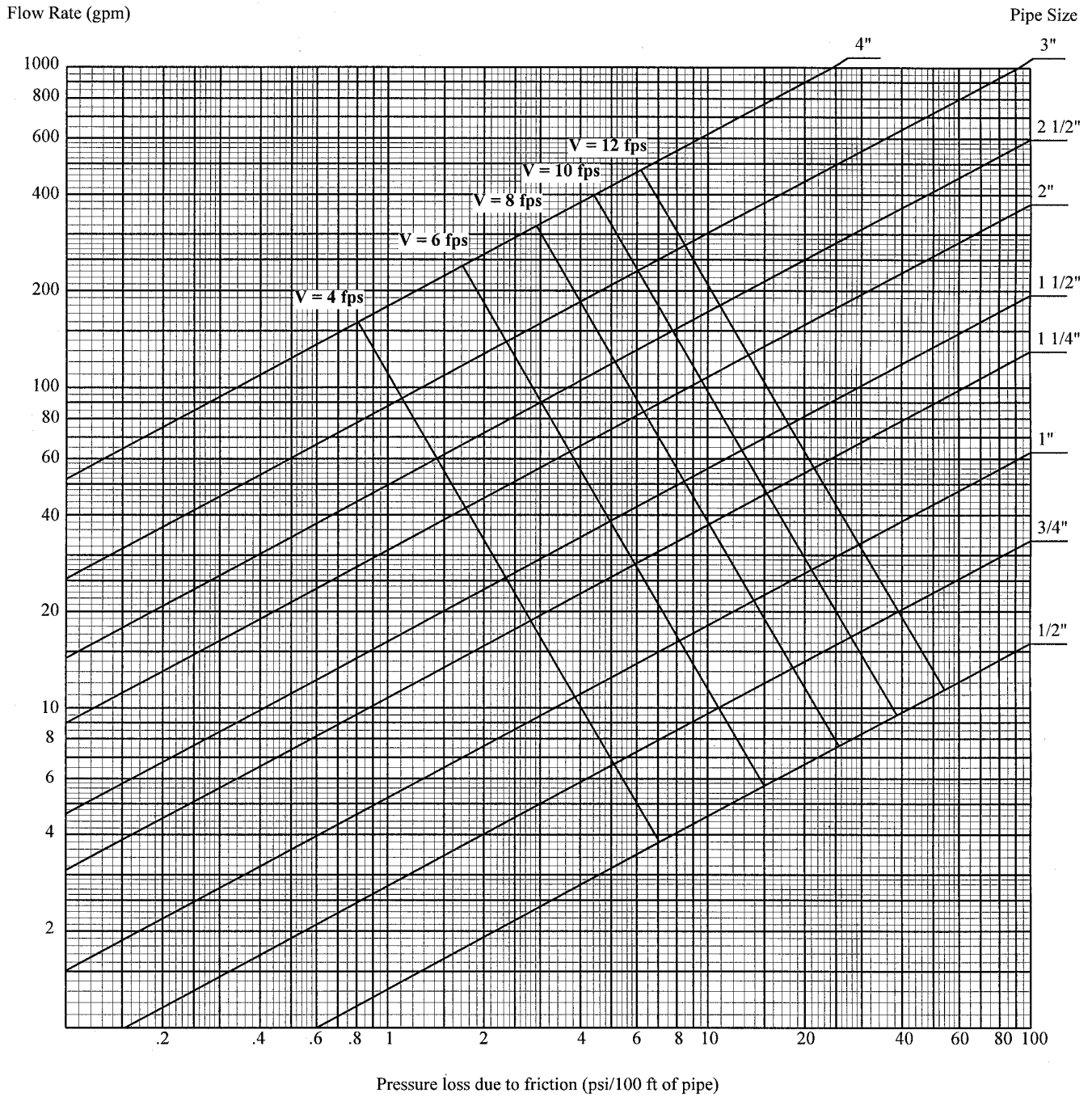
Graph A-382.40 (7)-4 PRESSURE LOSSES DUE TO FLOW FRICTION Material: Galvanized Steel Pipe-Schedule 40, ASTM A53, ASTM A120; (C = 125)
