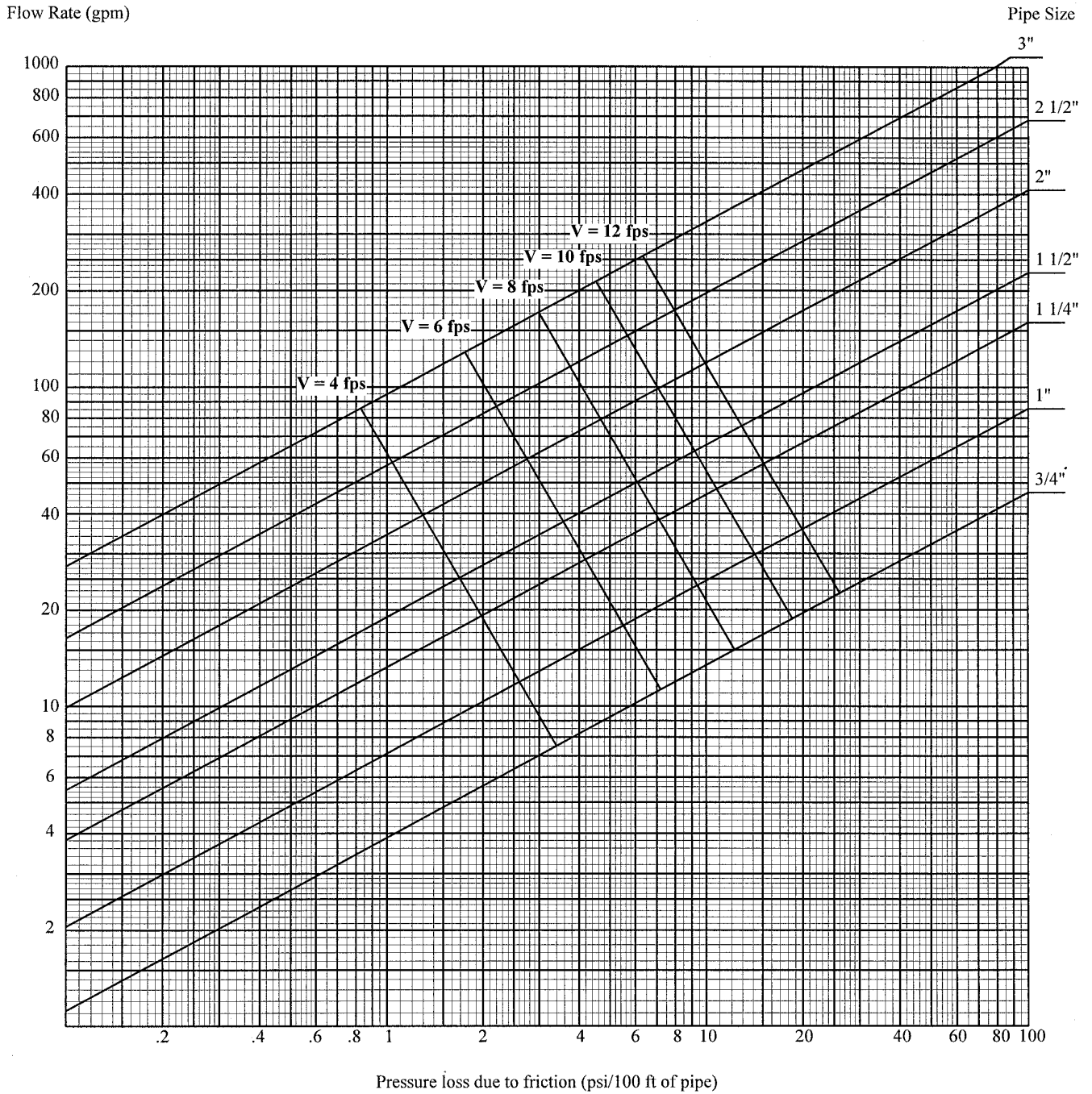
Graph A-382.40 (7)-11 PRESSURE LOSSES DUE TO FLOW FRICTION Material: CPVC Tubing, SDR 13.5; ASTM F442; (C = 150)
