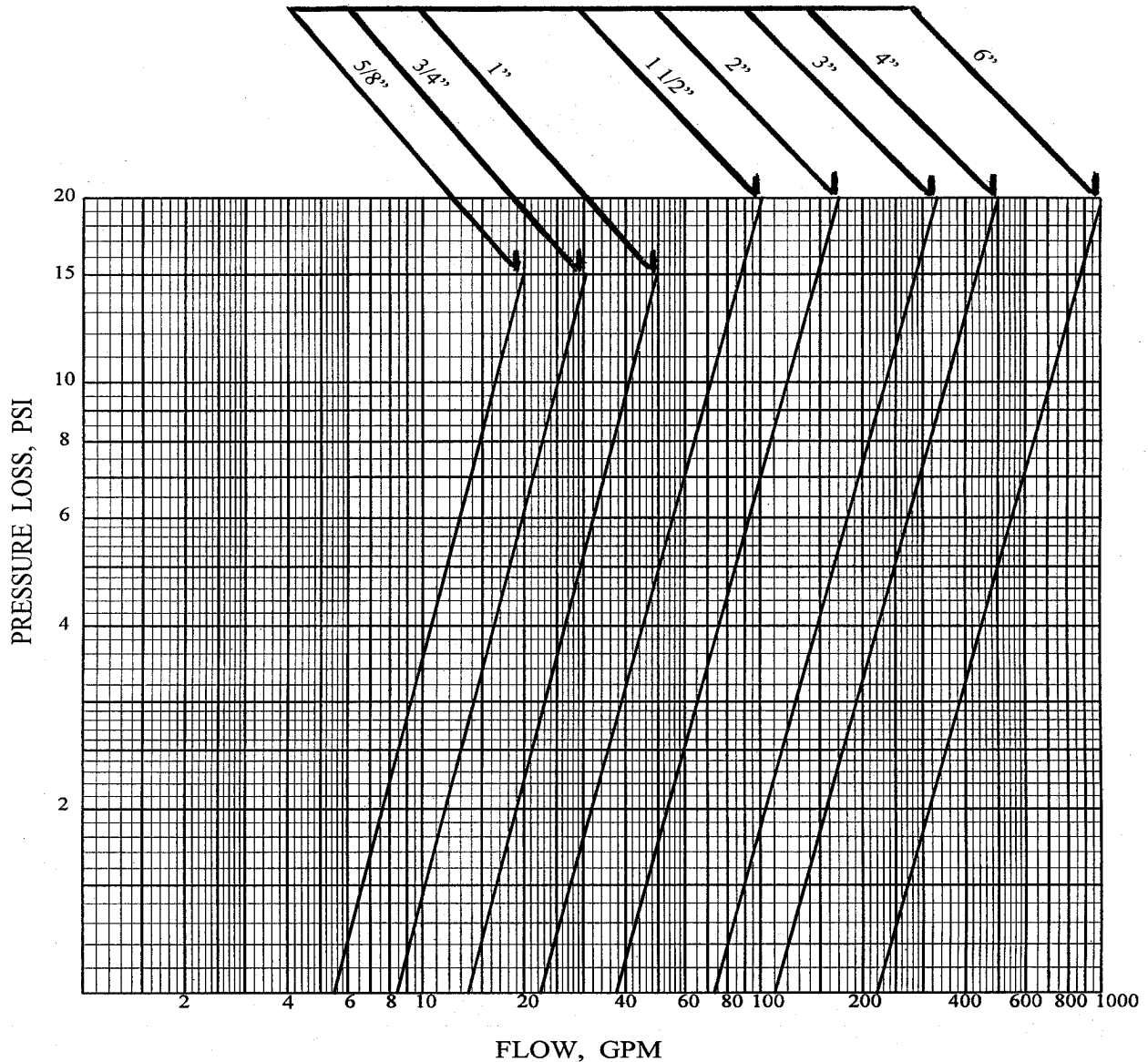
Graph A-382.40 (7)-1 PRESSURE LOSS IN COLD-WATER METERS, DISPLACEMENT TYPE MAXIMUM CAPACITY AND PRESSURE LOSS AS PER AWWA 6700-64
