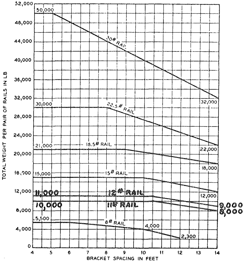
FIGURE 4.56 MAXIMUM WEIGHT OF CAR WITH RATED LOAD OR OF COUNTERWEIGHT WITH SAFETY FOR A PAIR OF GUIDE RAILS
