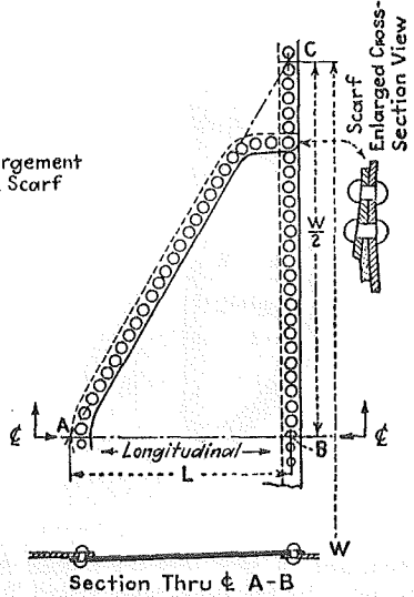
Fig. 3 Showing how patch may be shortened girthwise provided no more than 4 rivets are in a line parallel with the longitudinal seam.
