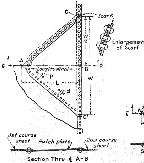
Fig. 4 DIAMOND SHAPE PATCH
