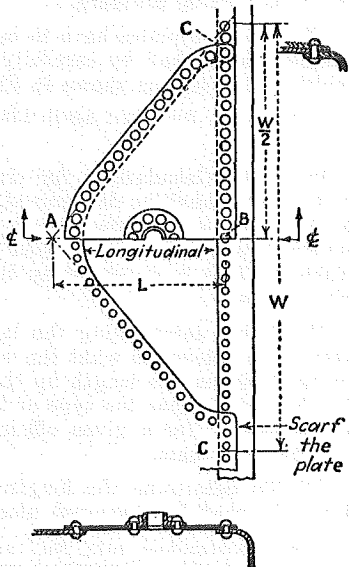
Fig. 5 TRIANGULAR PATCH
