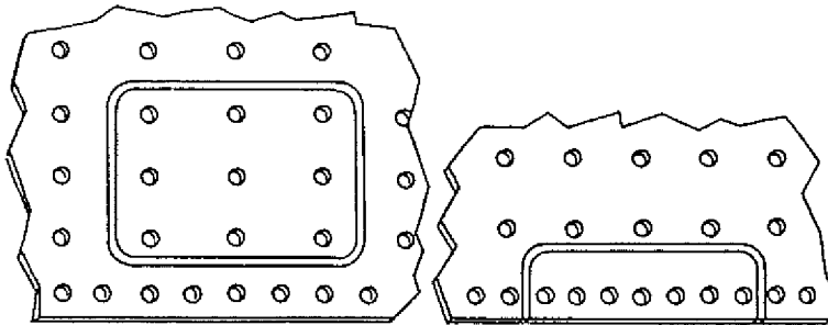
FLUSH PATCHES IN STAYED AREAS
