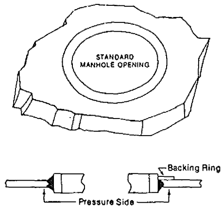
Figure 42.09-2 REPAIRS FOR ACCESS OPENINGS
