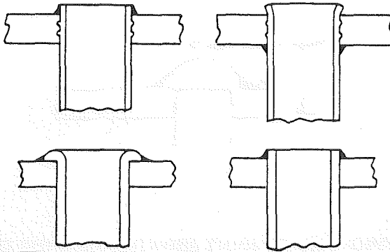
Figure 42.10-1 SEAL WELDING OF TUBES
