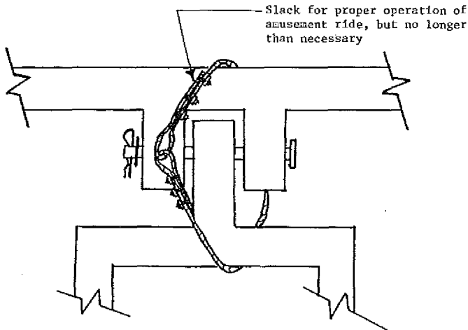
FIGURE 31.38-2 SAFETY CABLES
