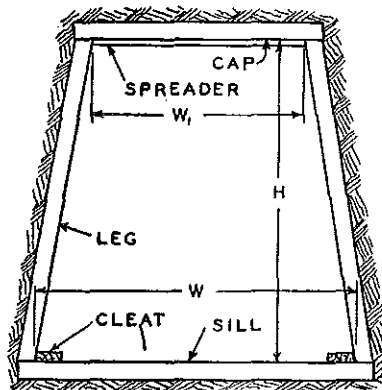
Fig. 3 Modified Box Type of Timbering
