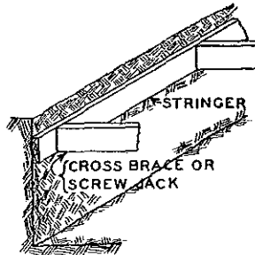
Fig. 13 Trench Timbering
