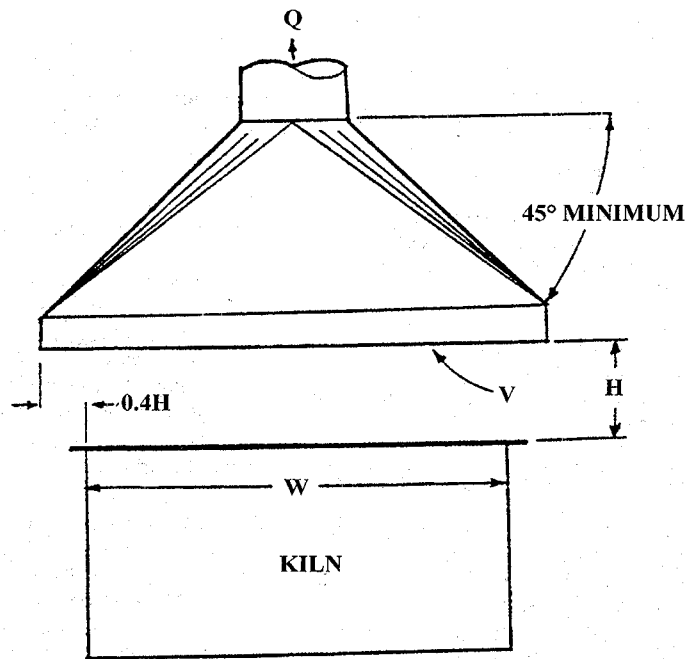
FIGURE 32.24 CANOPY HOOD
