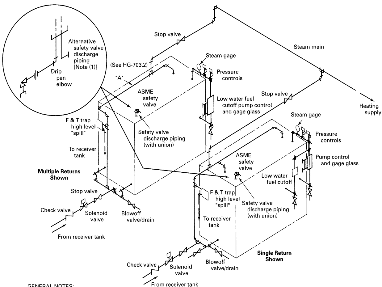
FIG. HG-703.1(a) STEAM BOILERS IN BATTERY — PUMPED RETURN — ACCEPTABLE PIPING INSTALLATION
