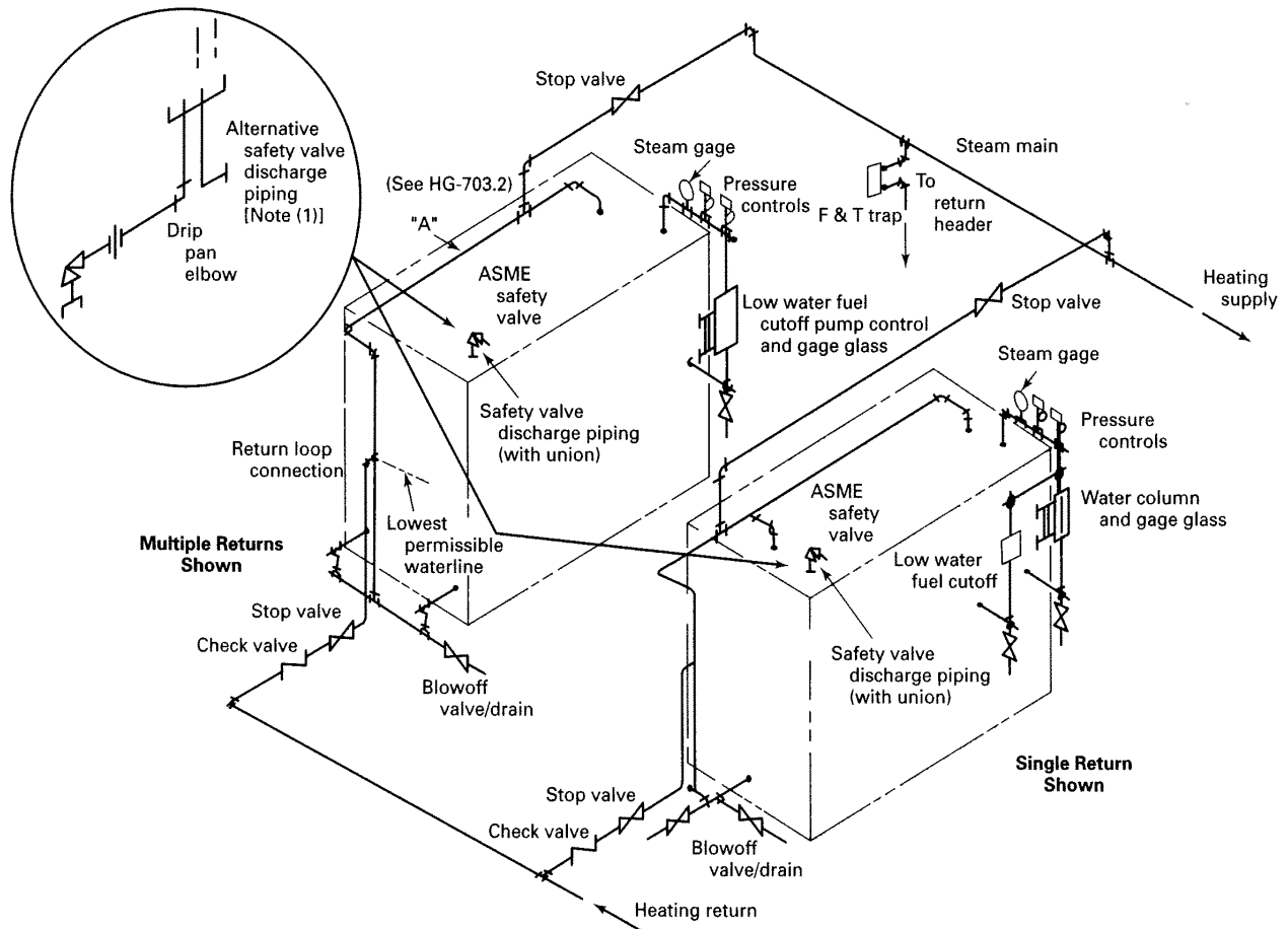
FIG. HG-703.1(b) STEAM BOILERS IN BATTERY – GRAVITY RETURN – ACCEPTABLE PIPING INSTALLATION
