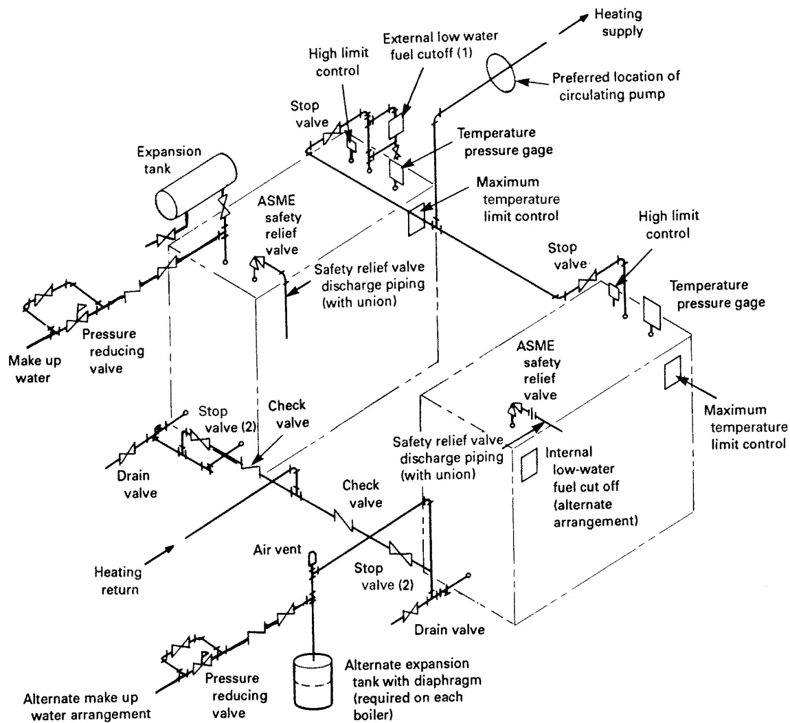
FIG. HG-703.2 HOT WATER BOILERS IN BATTERY — ACCEPTABLE PIPING INSTALLATION
