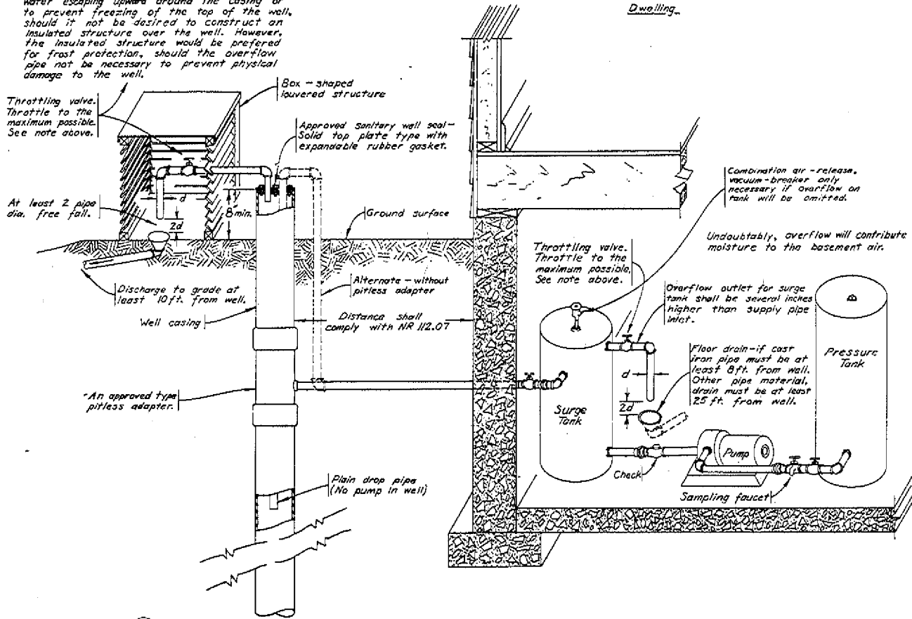
Figure ... Pump Installation for Flowing Well Showing alternatives of Above-Ground Discharge or a Approved Pitless Adapter Installation w/ Surge Tank and Booster Pump and Overflow Options at the Surge Tank or Top of the Well, if either is necessary.
