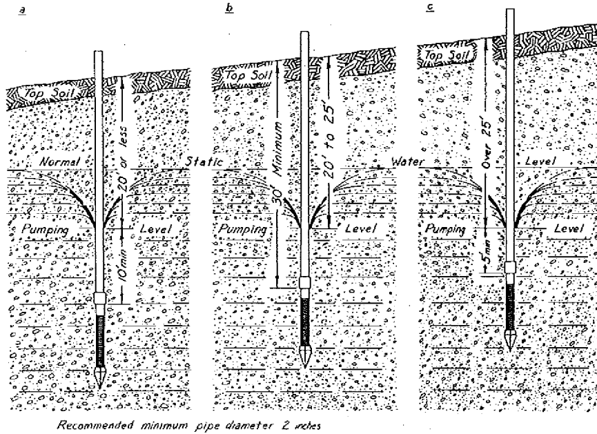
Figure 3. Construction of Driven-Point Wells in Sand and Gravel. See Table 1, a and NR 112.10.
