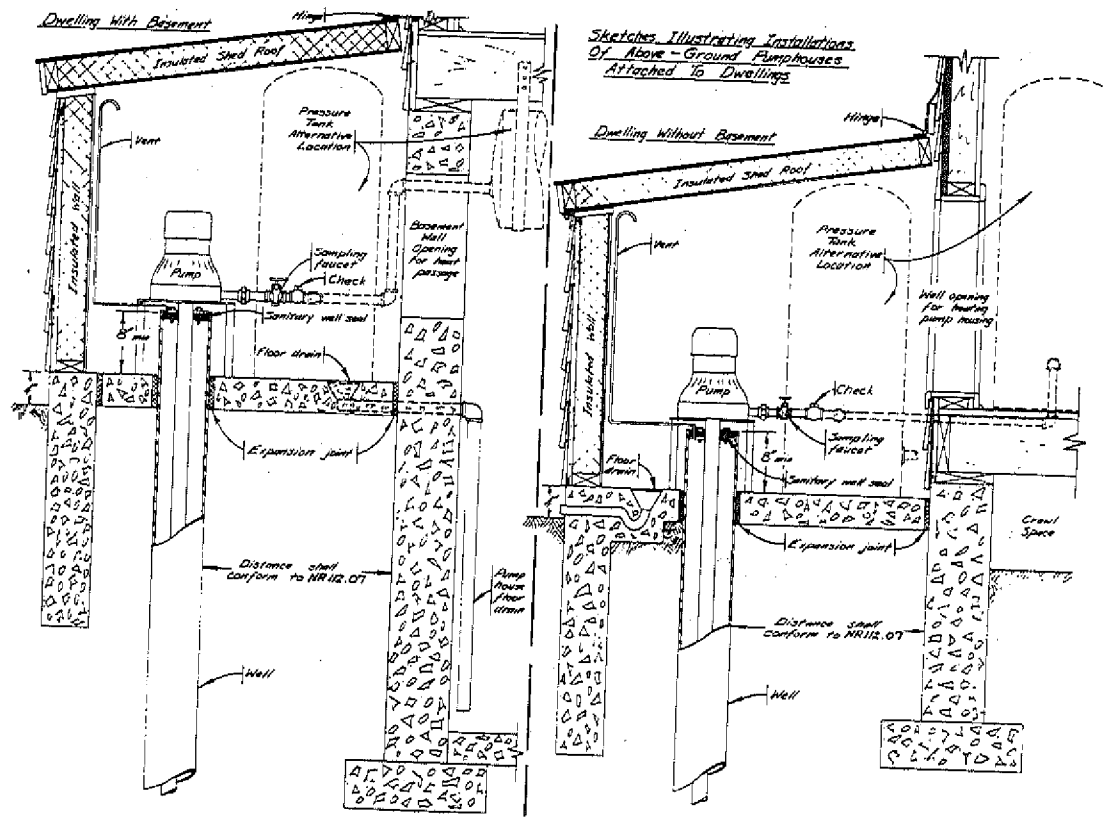
Figure 13. Insulated Pumphouse Adjoining a Dwelling.
