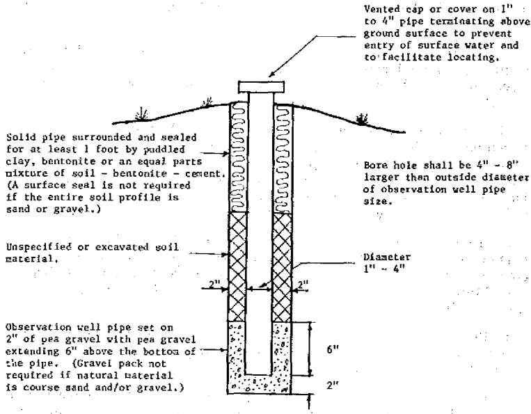
Figure 85.06 MONITORING WELL
