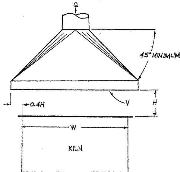
FIGURE 32.24 CANOPY HOOD
