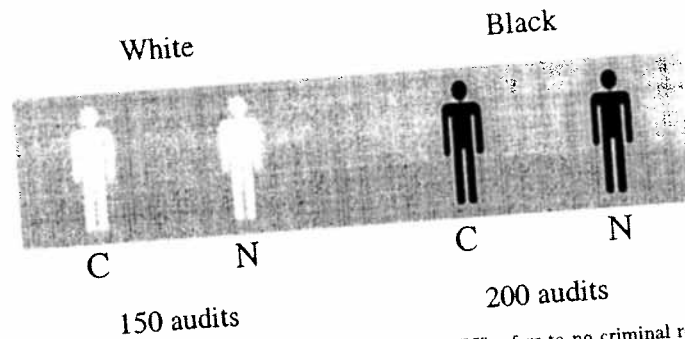
FIG. 3.—Audit design: "C" refers to criminal record; "N" refers to no criminal record
