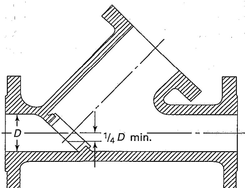
FIG. PG-60.3.7 Y-TYPE GLOBE VALVE
