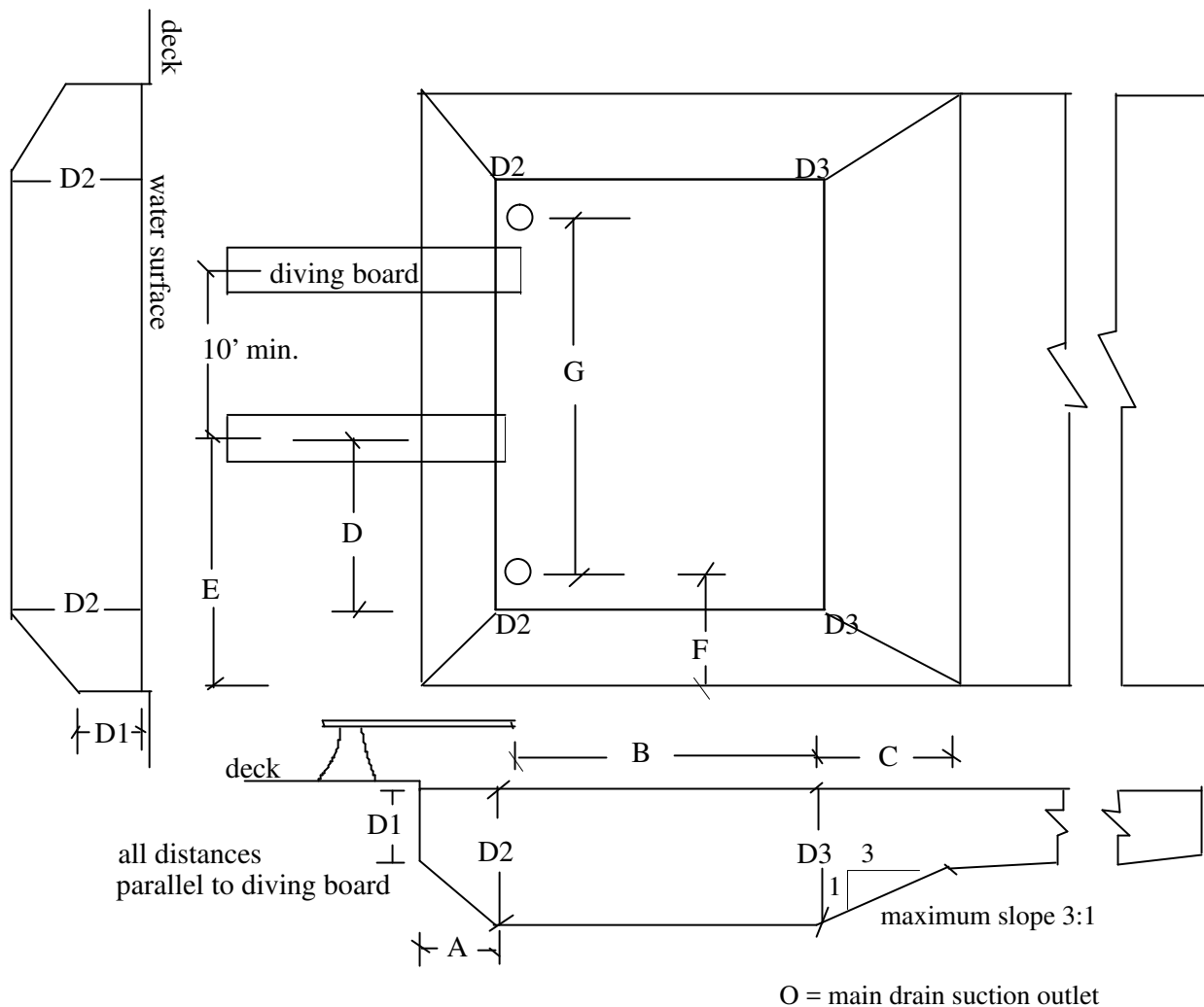
Figure 390.11-1 Diving Area Dimensions
