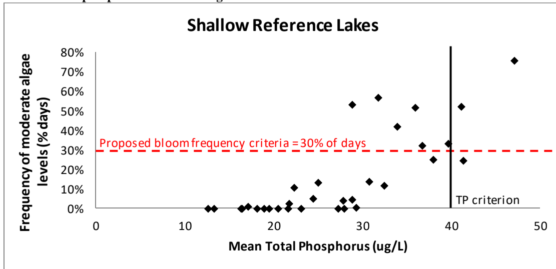
Figure 9. Statistically calculated frequency of summer moderate algae levels (chlorophyll a > 20 ug/L) in relation to mean total phosphorus levels among a set of shallow reference lakes.
