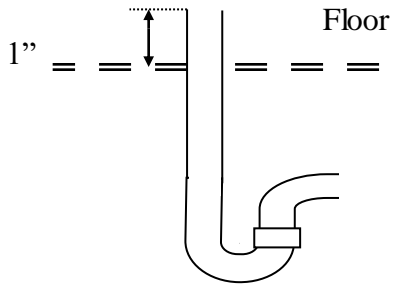
STANDPIPE IN
