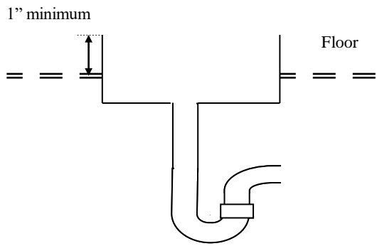
WASTE SINK IN
