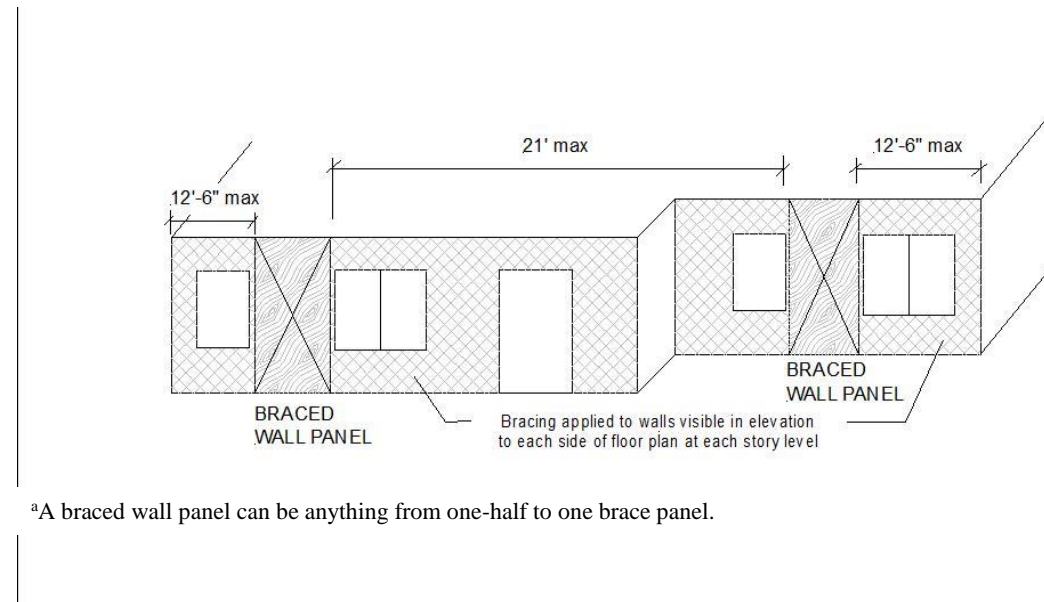
FIGURE 321.25–C LOCATION OF BRACED WALL PANELS ALONG A BUILDING SIDE a
