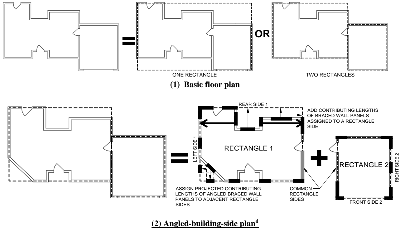
Figure 321.25–B DEFINING BUILDING SIDES AND LENGTHS WITH ONE OR MORE CIRCUMSCRIBED RECTANGLES a,b,c
