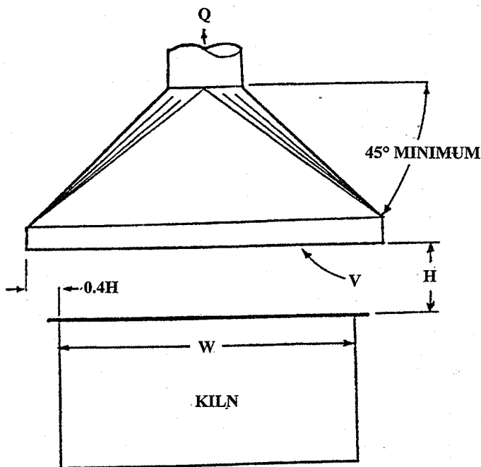
FIGURE 32.24 CANOPY HOOD
