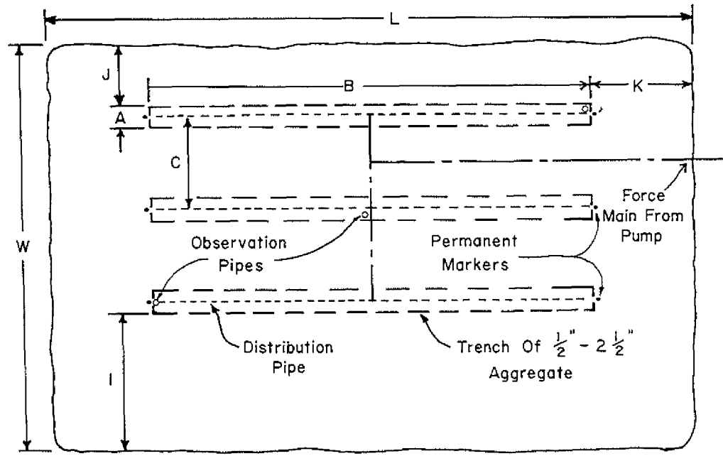
Mound Using 3 Trenches For Absorption Area
