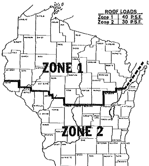
Zone Map for Roof Loads
