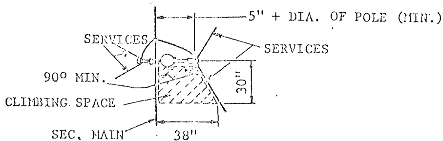
Figure PSC 114-236J. Climbing Space Past Rack Construction
