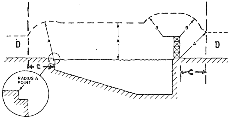
Swimming Pool Clearances
