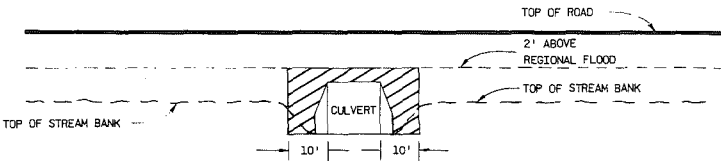
END VIEW
