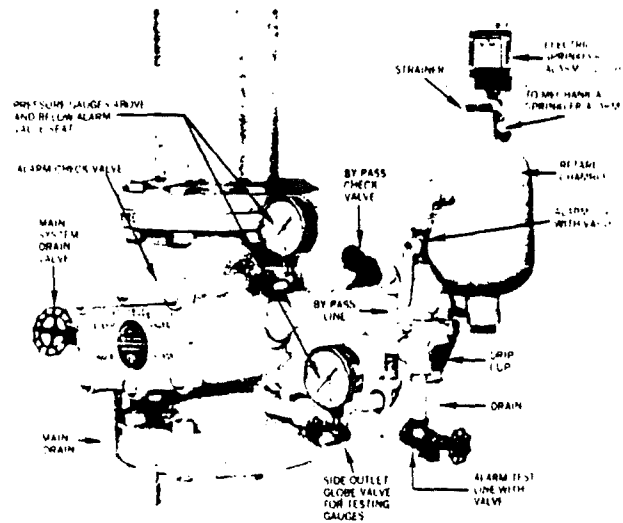
Figure 1-3(d) Typical alarm valve and trimmings.
