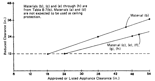
Figure 8-7(g) Ceiling Protection Using Materials in Table 8-7(b).
