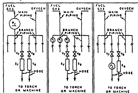
Fig. Q-1 Fig. Q-2 Fig. Q-3 LEGEND P f — Protective equipment in fuel gas piping V f — Fuel gas station outlet valve V o — Oxygen station outlet valve B f — Backflow prevention device(s) at fuel gas station outlet B o — Backflow prevention device(s) at oxygen station outlet
