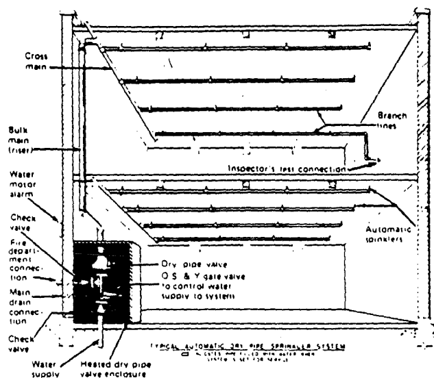
Figure 1-3(a) Dry-pipe system.
