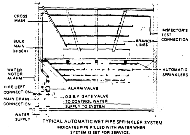
Figure 1-3(c) Wet-pipe system.
