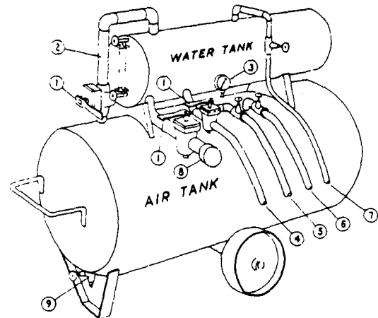
Figure 5-13.5.1 Hydropneumatic Machine.
