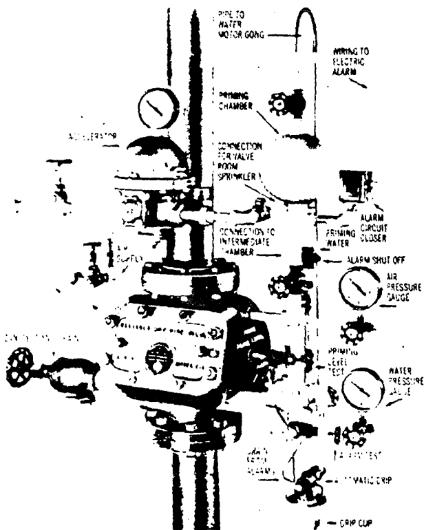
Figure 1-3(b) Typical dry-pipe valve with trimmings.
