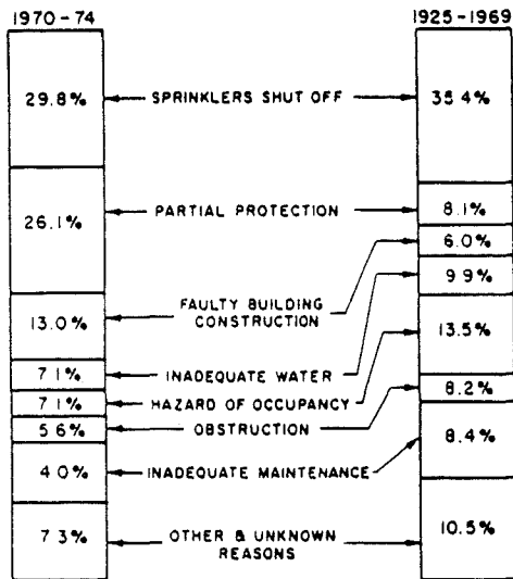
Figure 7-2.1 Reasons for unsatisfactory sprinkler system performance.
