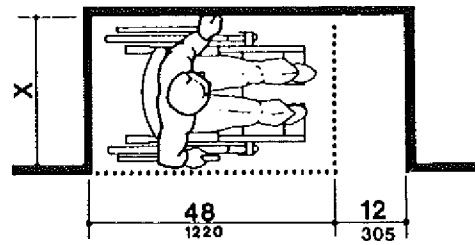
(e) Additional Maneuvering Clearances for Alcoves
