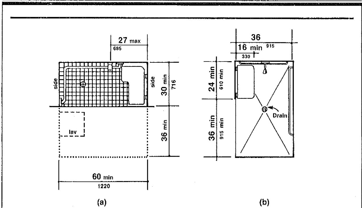
Fig. 57 Roll-in Shower with Folding Seat
