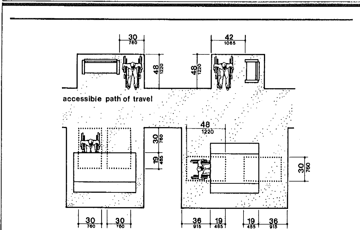
Fig. 45 Minimum Clearances for Seating and Tables
