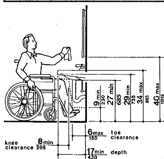
Fig. 31 Lavatory Clearances
