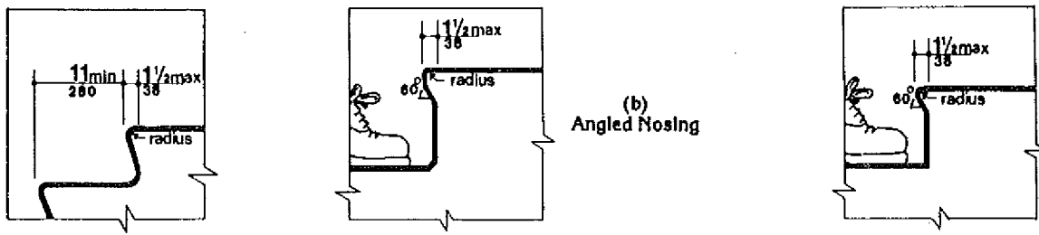
(a) Flush Riser (b) Angled Nosing (c) Rounded Nosing Fig. 18 Usable Tread Width and Examples of Acceptable Nosings
