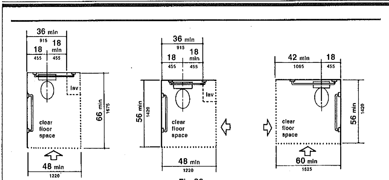
Fig. 28 Clear Floor Space at Water Closets
