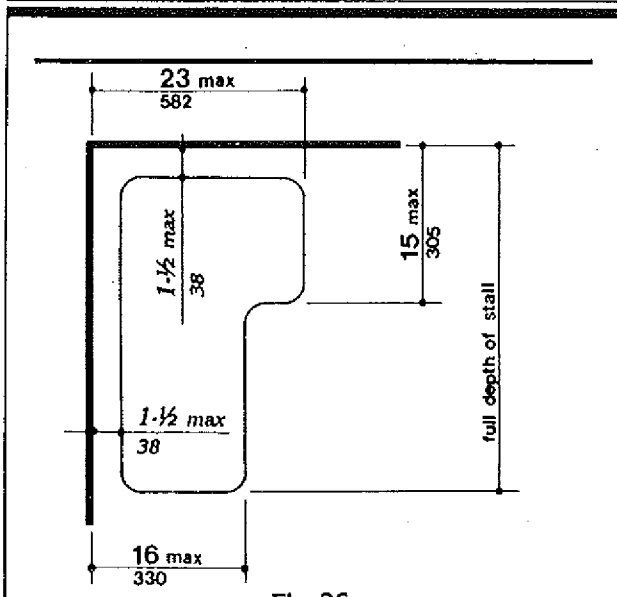
Fig. 36 Shower Seat Design
