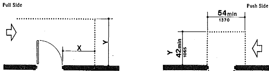
(a) Front Approaches — Swinging Doors
