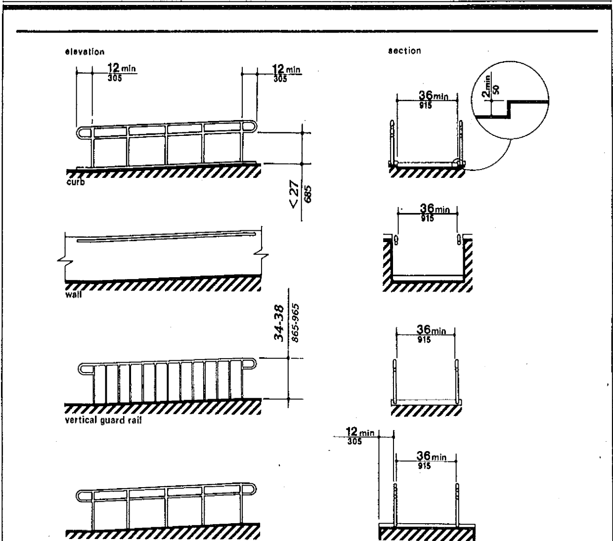
Fig. 17 Examples of Edge Protection and Handrail Extensions
