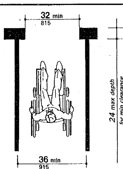
Fig. 1 Minimum Clear Width for Single Wheelchair
