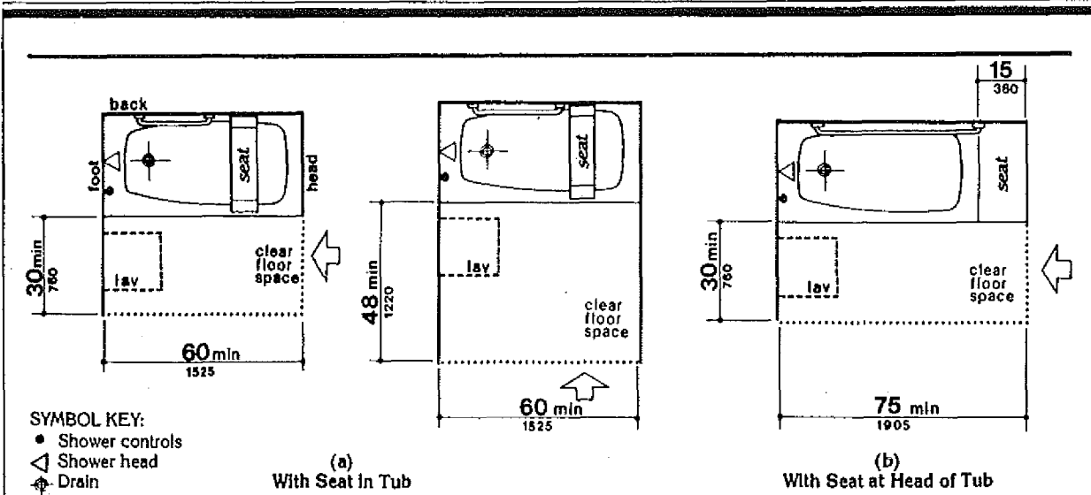
Fig. 33 Clear Floor Space at Bathtubs
