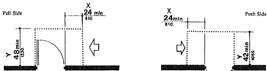
(b) Hinge Side Approaches — Swinging Doors
