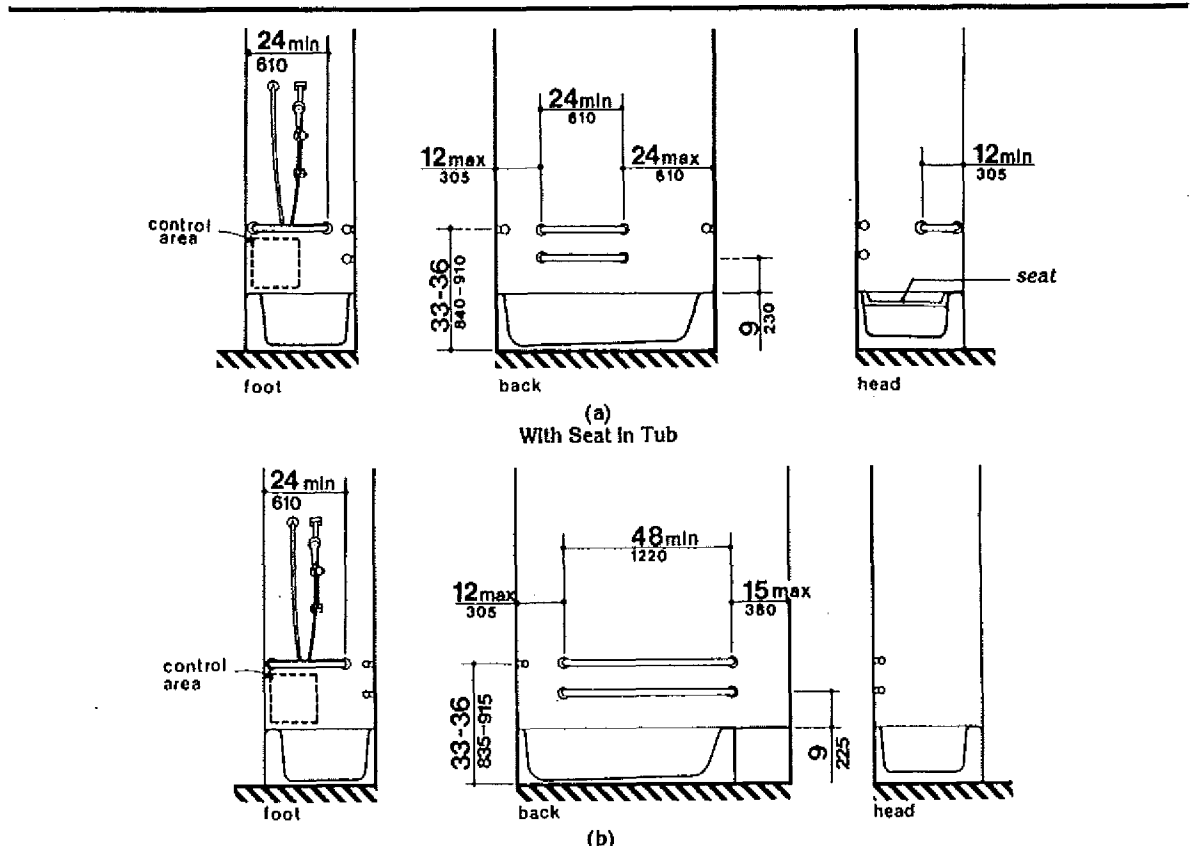
Fig. 34 Grab Bars at Bathtubs
