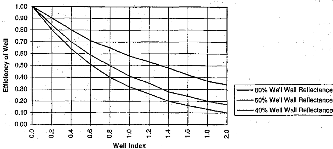
Figure 63.02 Well Efficiency
