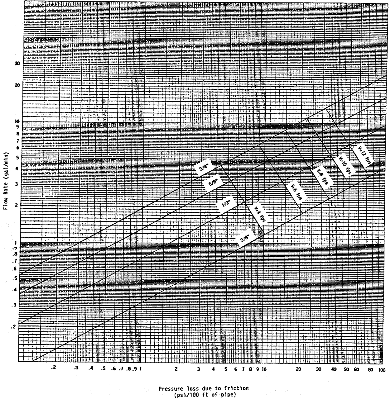
Graph A-82.40 (7)-6 Pressure losses due to flow friction Material: Crosslinked Polyethylene (PEX) Tubing, ASTM F876
