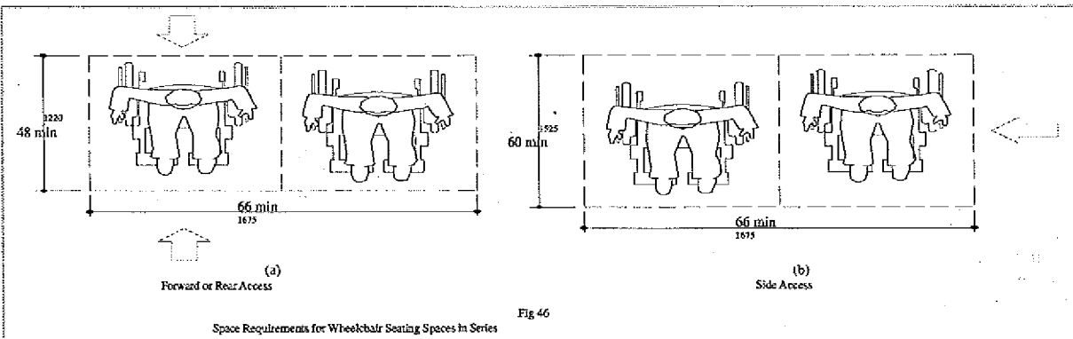
Fig 46 Space Requirements for Wheelchair Seating Spaces in Series
