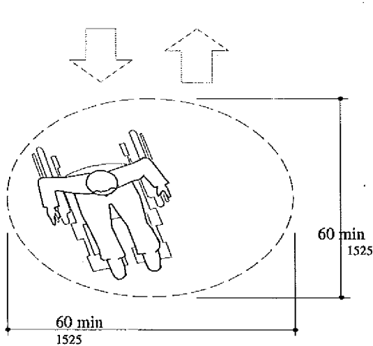
(a) 60-IN. (1525-MM.) Diameter Space
