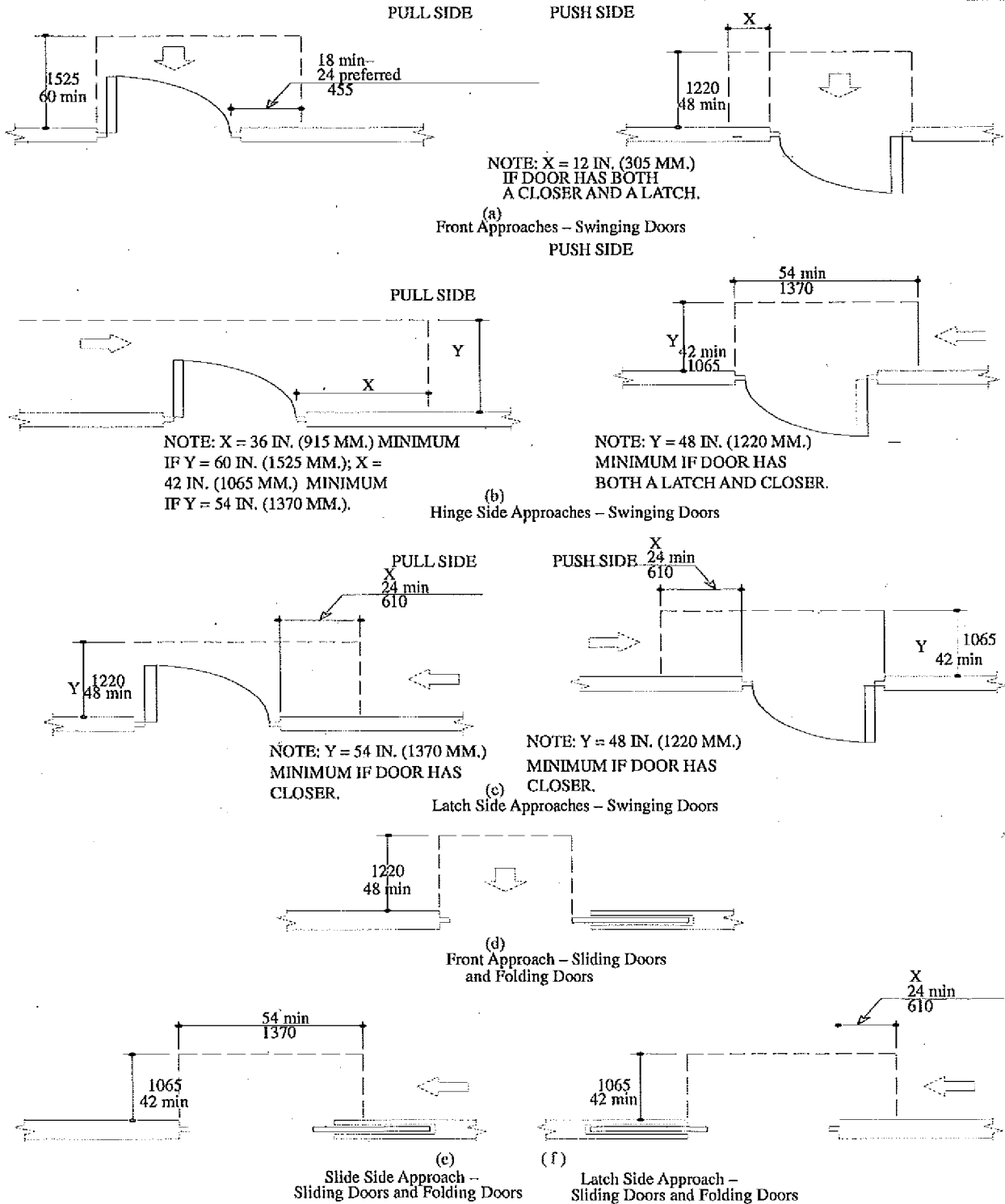
Fig 25 Maneuvering Clearance at Doors
