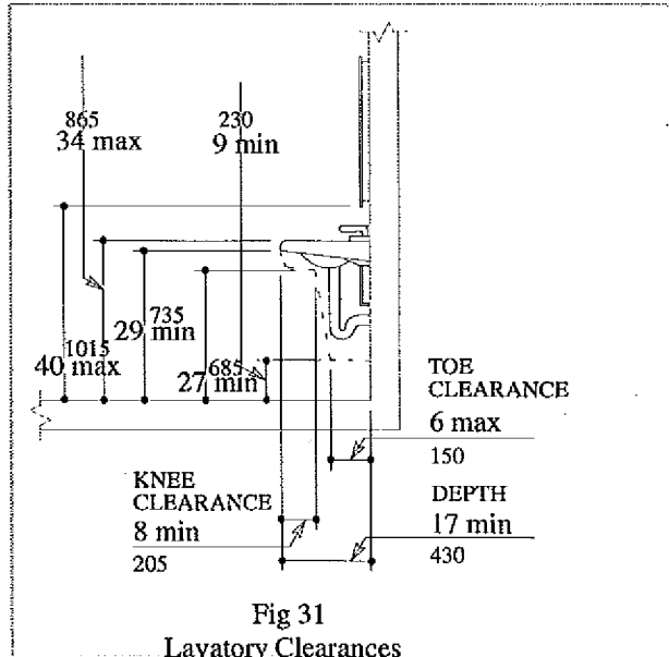
Lavatory Clearances
