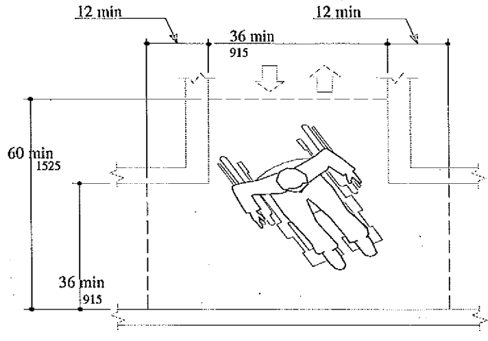
(b) T-Shaped Space for 180 Degree Turns
