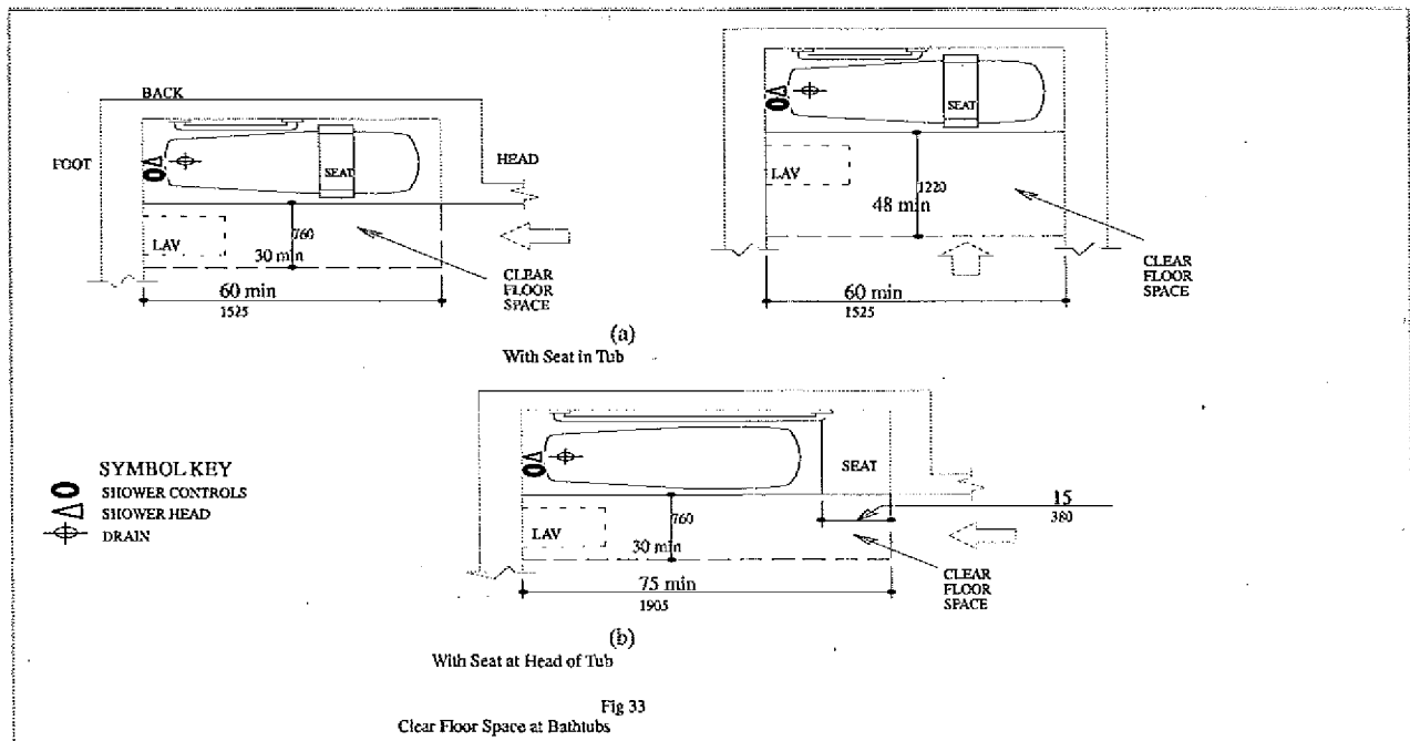
Clear Floor Space at Bathtubs
