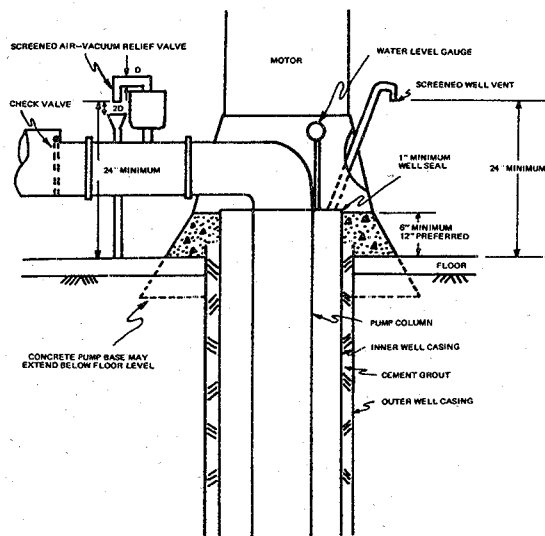
TYPICAL WELL PUMP INSTALLATION - PUBLIC SUPPLY WELLS
