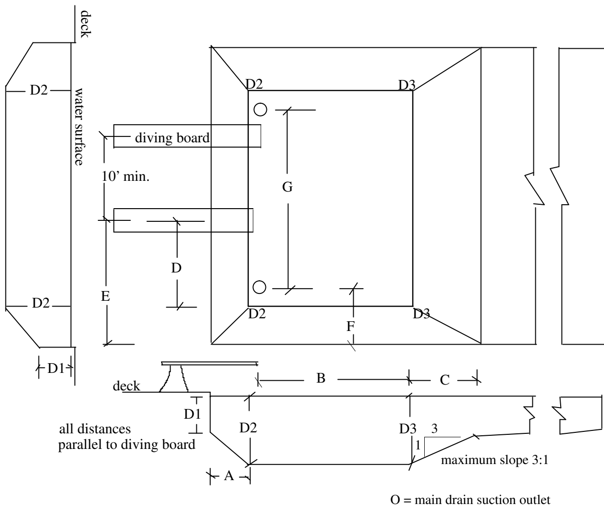
Figure 90.11-1 Diving Area Dimensions
