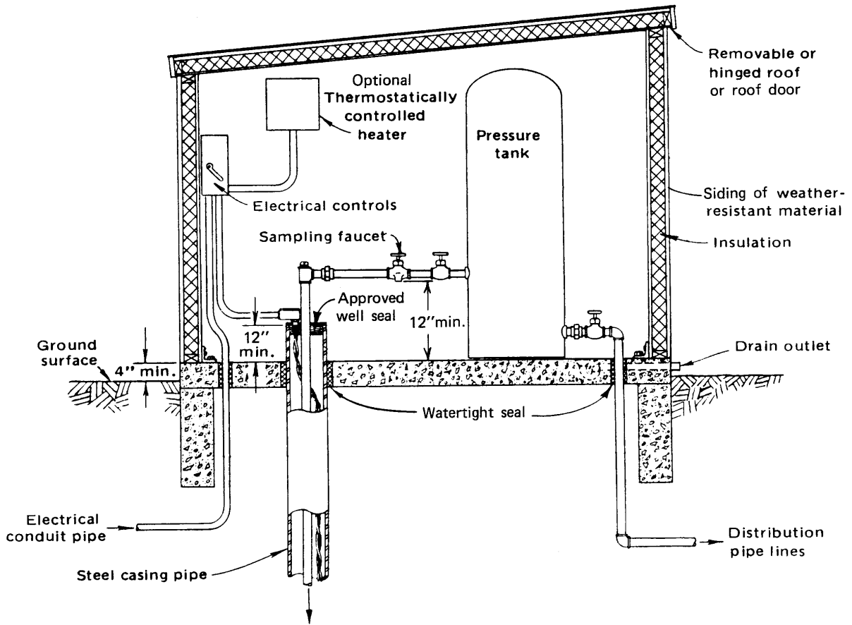
Figure 46. Pumphouse specifications.
