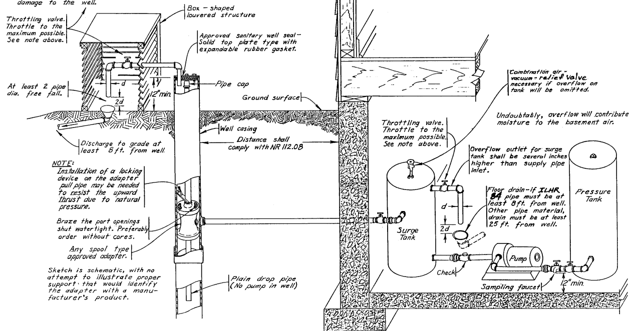
Figure 43. Overflow piping arrangement for a flowing well with a surge tank and with no pump.
