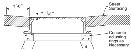
Adjusting utility cover level with road.
