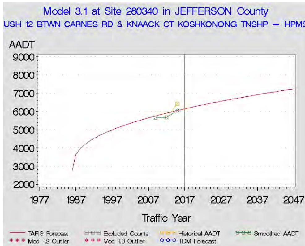
Figure 30.2.4: Model 3.1 Graphical Output at a Traffic Site in Jefferson County
