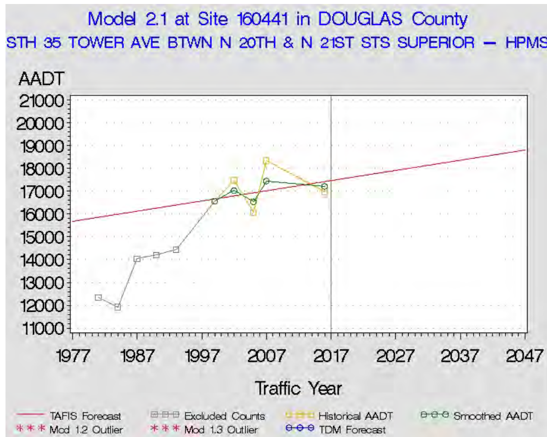
Figure 30.2.2: Model 2.1 graphical output at a traffic site in Douglas County
