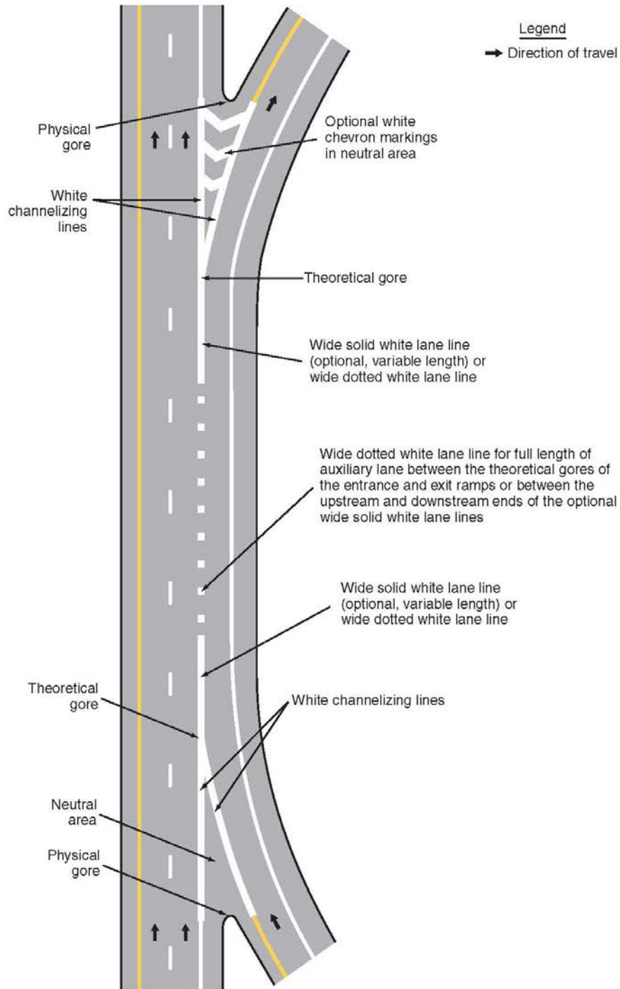
Figure 3B-10. Examples of Applications of Freeway and Expressway Lane-Drop Markings (Sheet 5 of 5)
