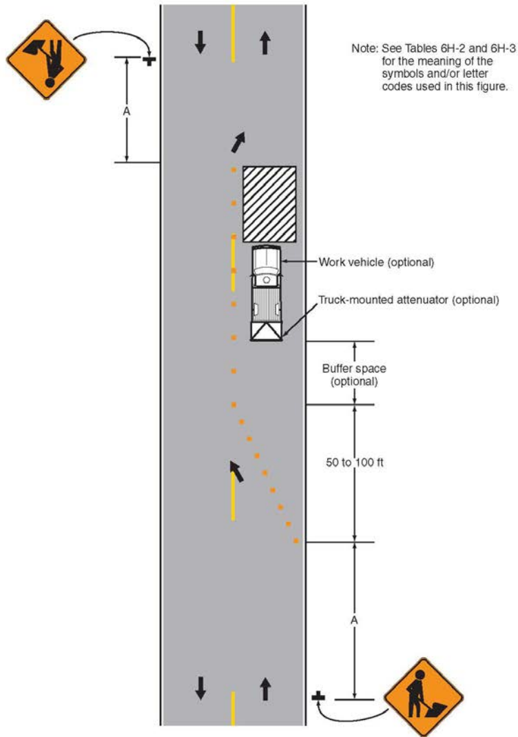
Typical Application 18
