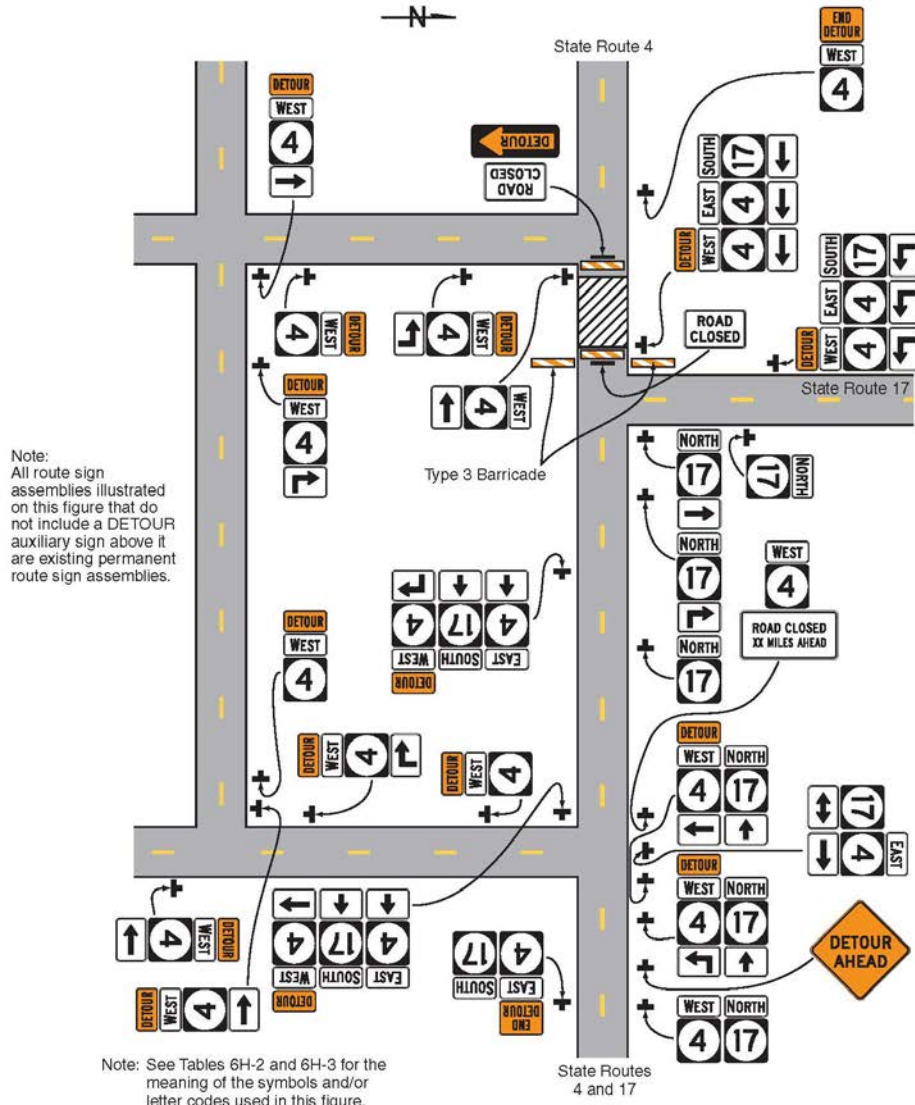
Typical Application 9
