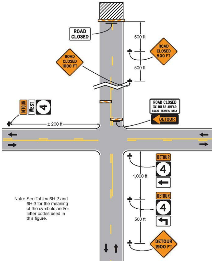
Typical Application 8
