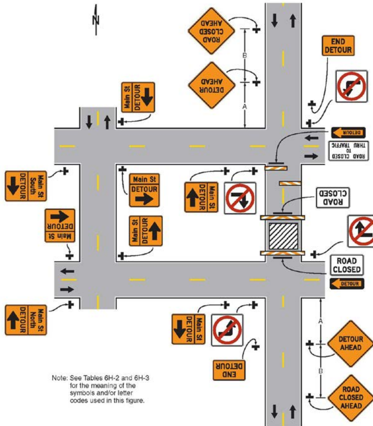
Figure 6H-20. Detour for a Closed Street (TA-20)
