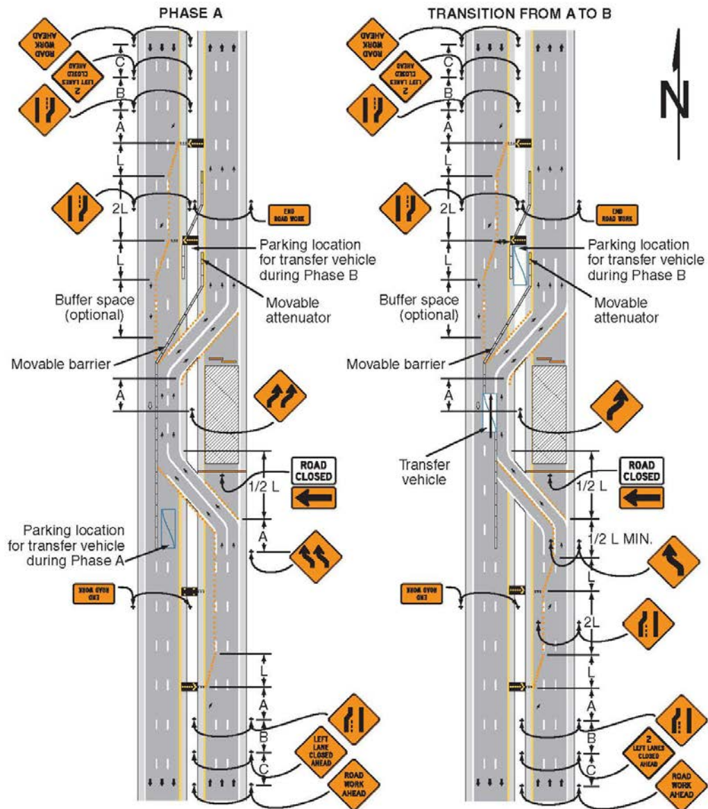
Typical Application 45
