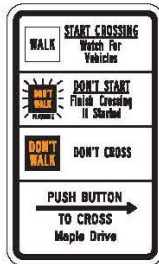
R10-3g
