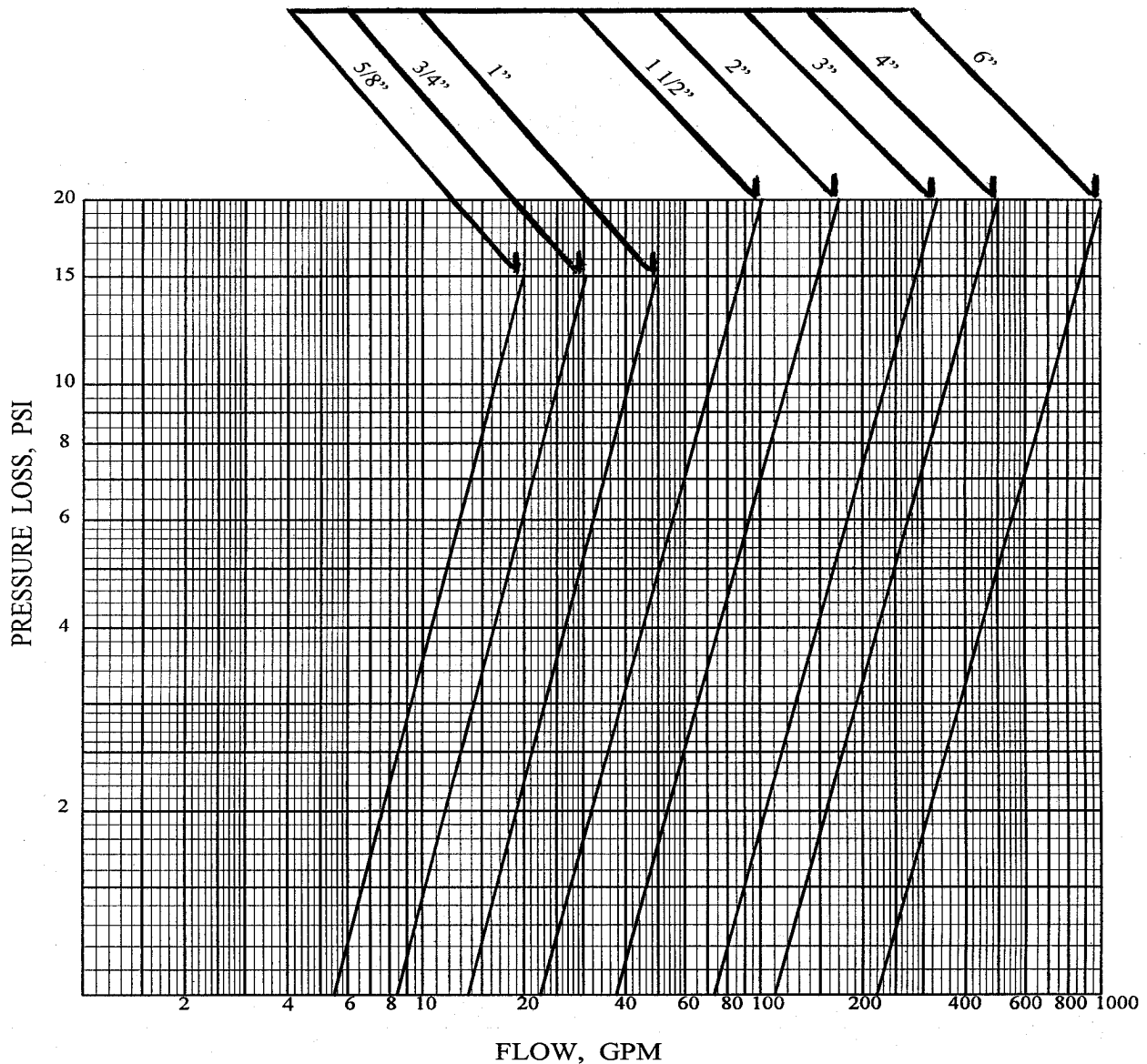
Graph A-382.40 (7)-1 PRESSURE LOSS IN COLD-WATER METERS, DISPLACEMENT TYPE MAXIMUM CAPACITY AND PRESSURE LOSS AS PER AWWA 6700-64
