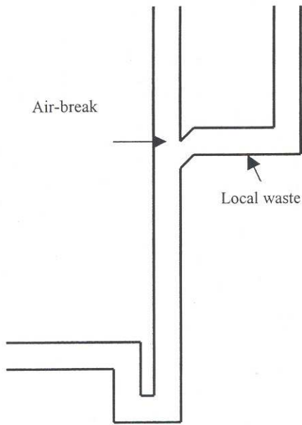
LOCAL WASTE DISCHARGING TO STANDPIPE
