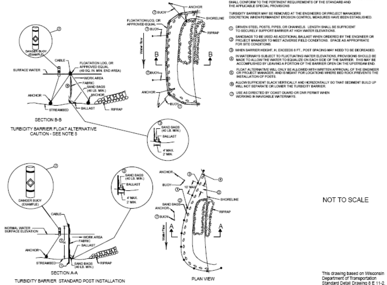
Figure 1. Turbidity Barrier Placement Details
