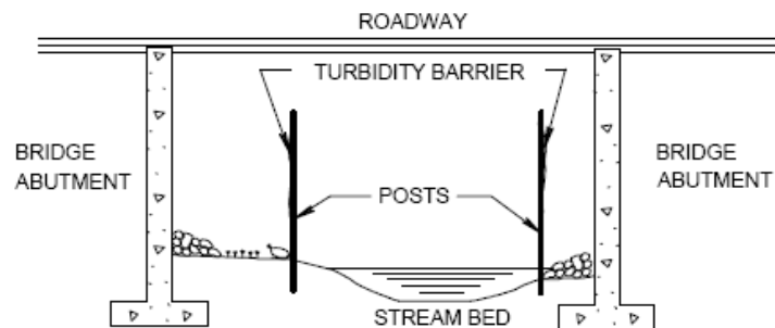
SECTION C-C
