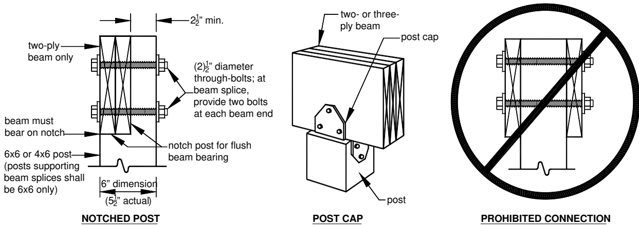
Figure 2 POST-TO-BEAM CONNECTIONS
