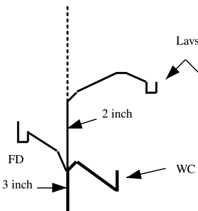
Individual vent serving as a wet vent
