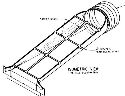
GRATES FOR HORIZONTAL PIPING
