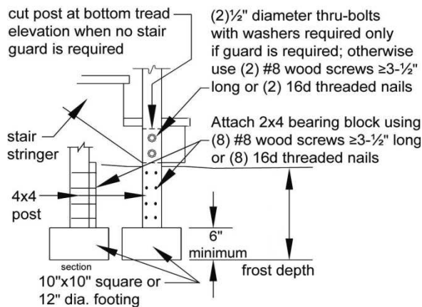
Figure 29 STRINGER BEARING
