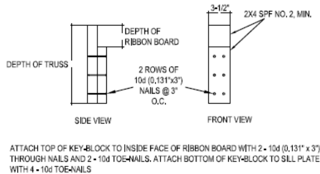
Detail 1: Attachment of Deck Ledger to Floor System with MPCW Trusses
