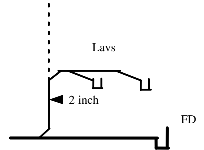
Common vents serving as a wet vent
