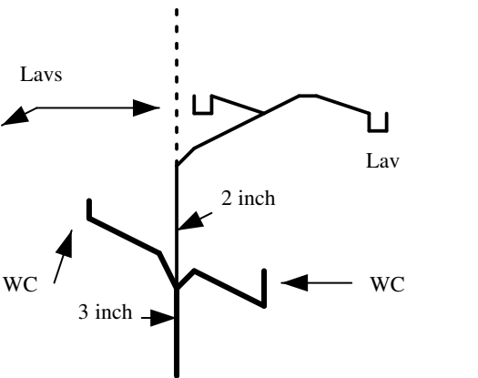
Common vents serving as a wet vent
