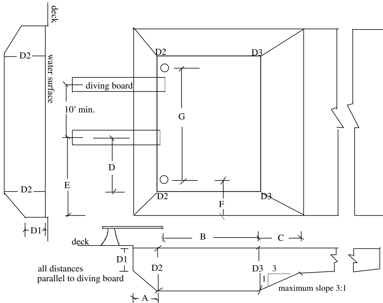
Figure 390.11–1 Diving Area Dimensions
