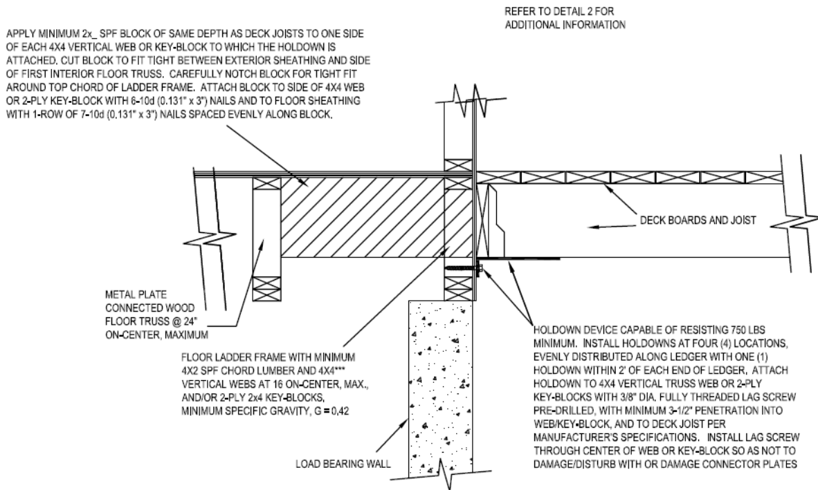
Detail 3: Deck Lateral Load Connection Capable of Resisting the 1500 lbf Lateral Load Requirement
